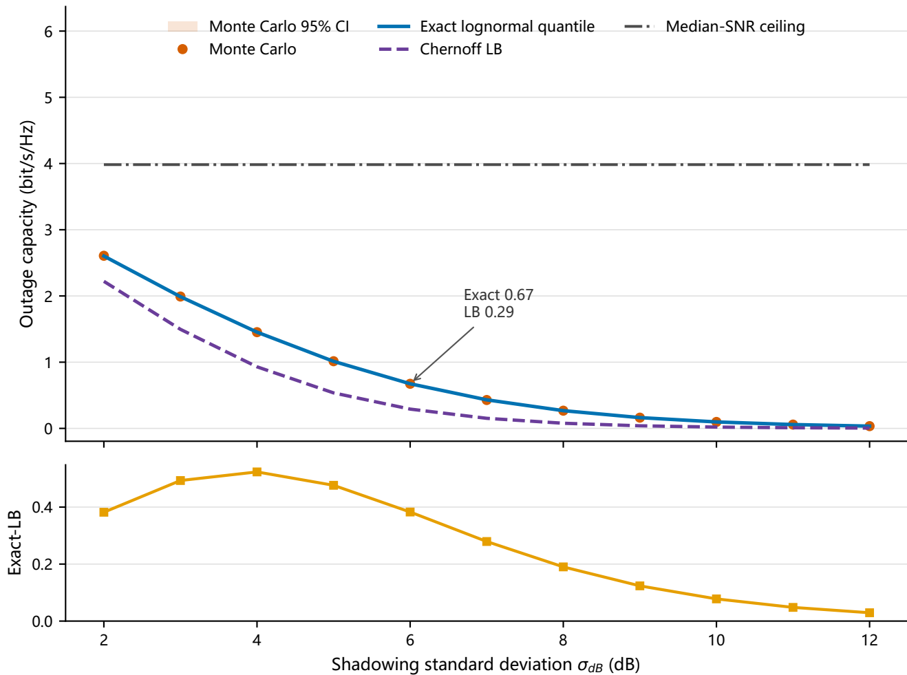
Theory--simulation comparison, \varepsilon = 10^{-2} , GEO S-band \gamma_0 = 11.71 dB
