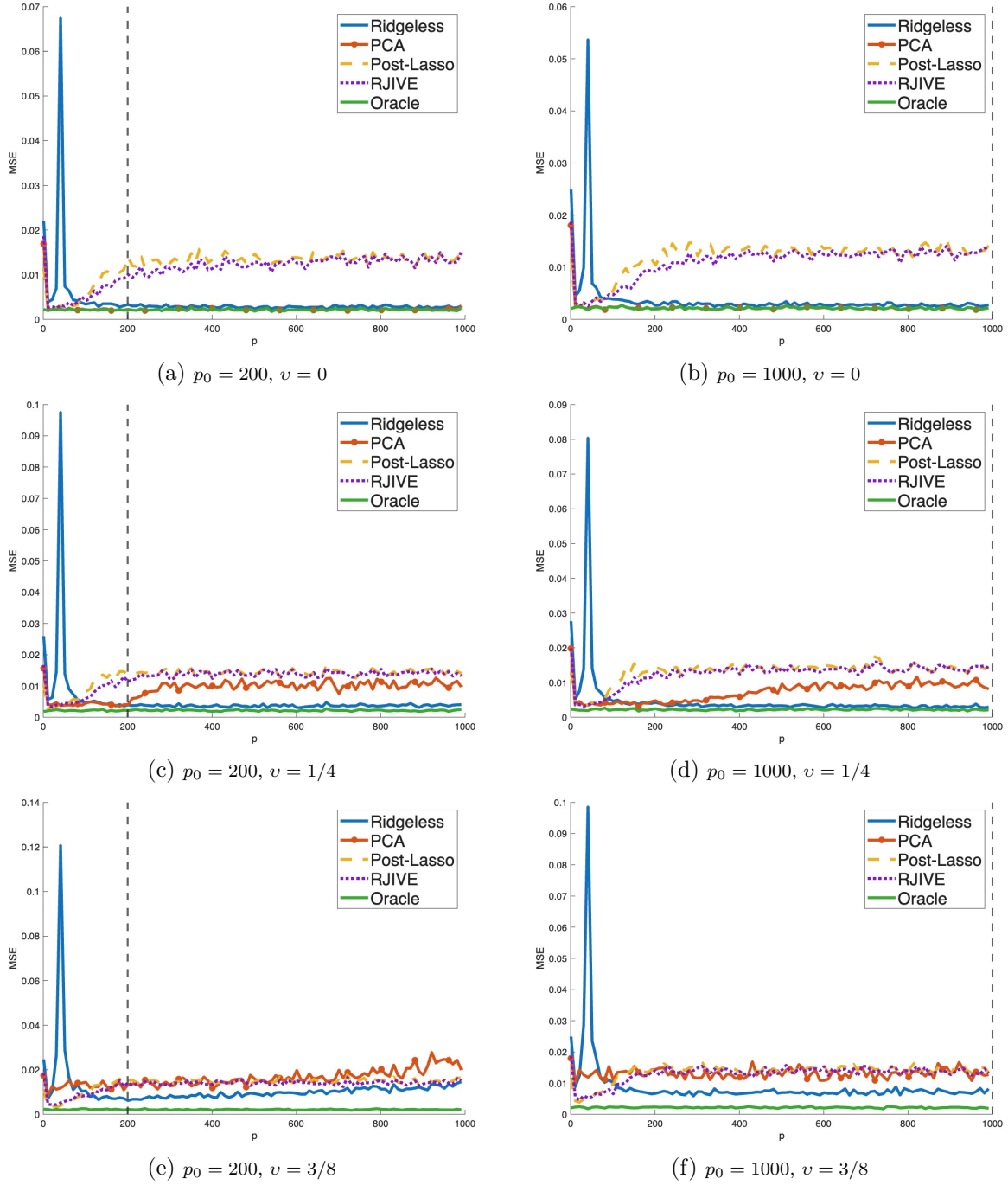
Figure 2: MSEs of \hat{\alpha} as the number of instruments p increases. All estimation methods use the full set of instruments. The vertical dashed line indicates the maximum number of informative instruments p_0 . Each subplot corresponds to a different factor strength v and maximum number of informative instruments p_0 , respectively. All results are based on 100 simulation replications and sample size n = 100 .
