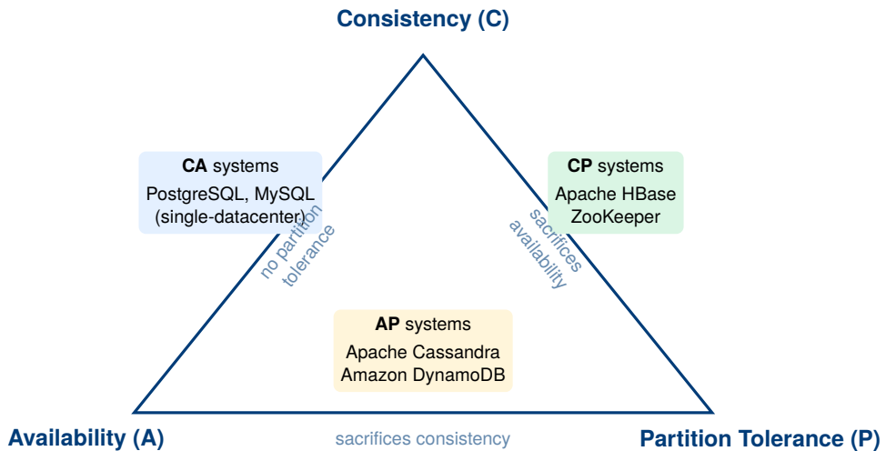
Figure 1.1: The CAP triangle: every distributed system chooses two of the three properties. Because network partitions are unavoidable, real systems choose between CP and AP.
