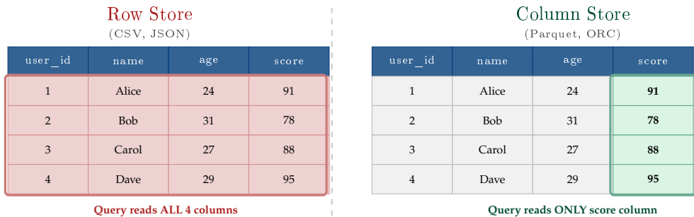
Figure 5.2: Row-oriented vs. columnar storage for a SELECT score FROM users query. The row store reads all four columns for every row (red box). The column store reads only the score column chunk (green box), skipping user_id , name , and age entirely. For 100 columns with a 3-column query, the columnar store provides a 33× I/O reduction.
