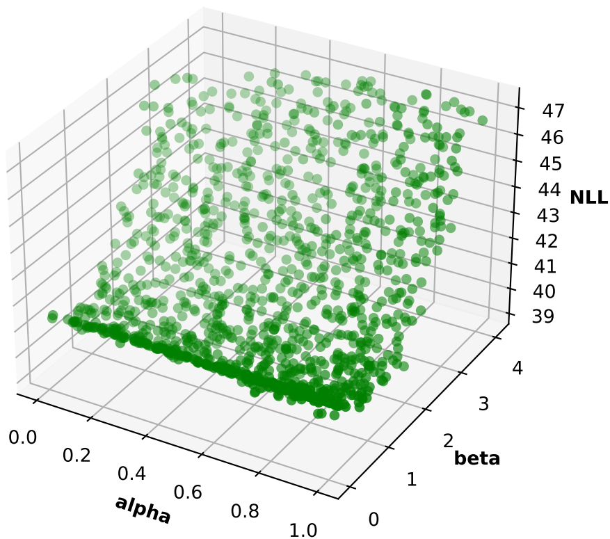
Participant 01, run 2: NLL, alpha and beta 3D scatter plot
