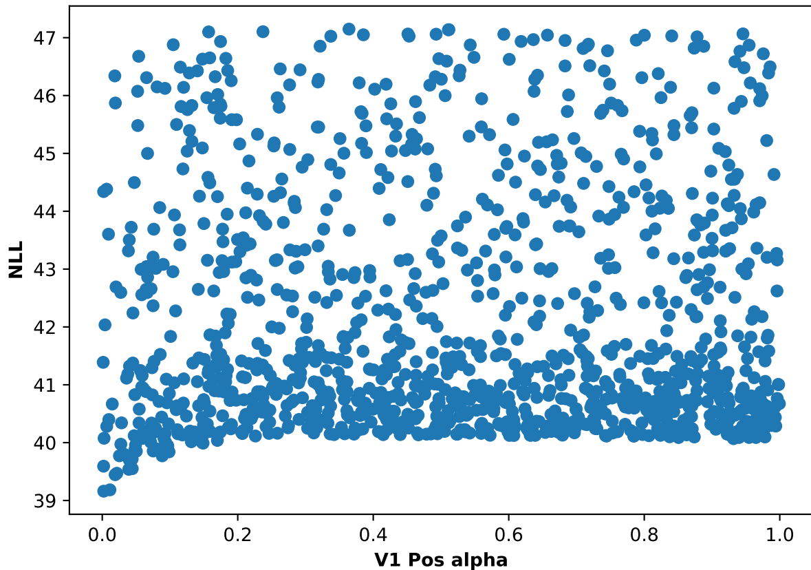
Participant 01, run 2: NLL and V1 Pos alpha scatter plot
