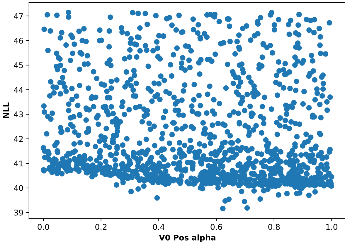
Participant 01, run 2: NLL and V0 Pos alpha scatter plot
