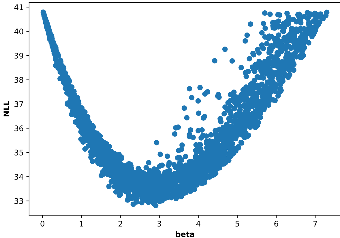
Participant 01, run 3: NLL and beta scatter plot
