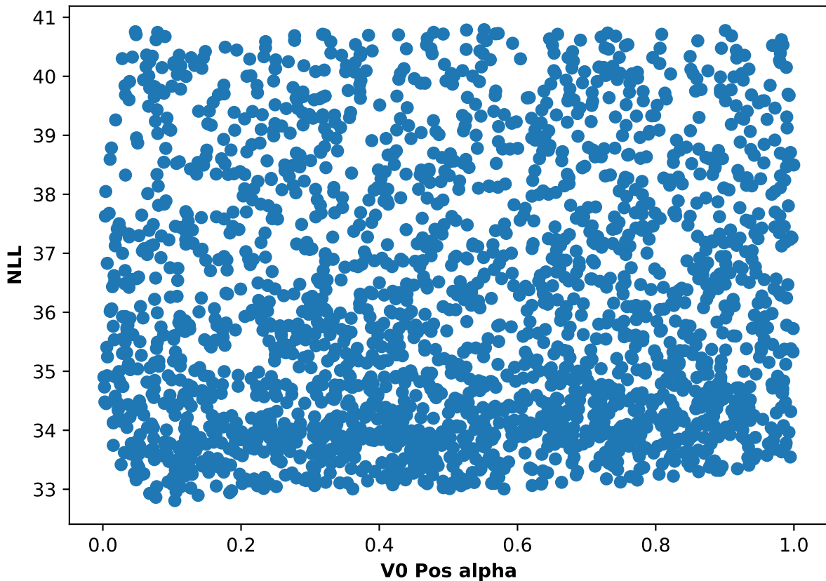
Participant 01, run 3: NLL and V0 Pos alpha scatter plot
