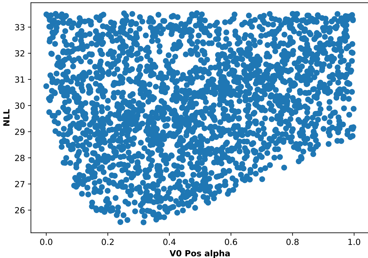
Participant 02, run 2: NLL and V0 Pos alpha scatter plot
