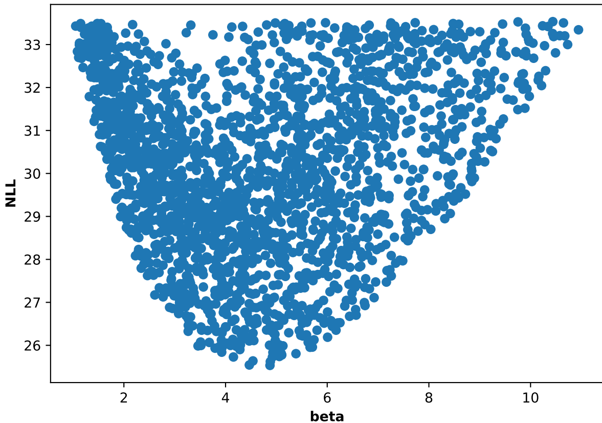
Participant 02, run 2: NLL and beta scatter plot
