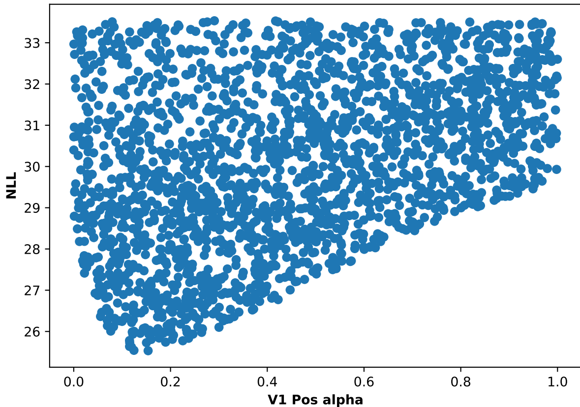
Participant 02, run 2: NLL and V1 Pos alpha scatter plot
