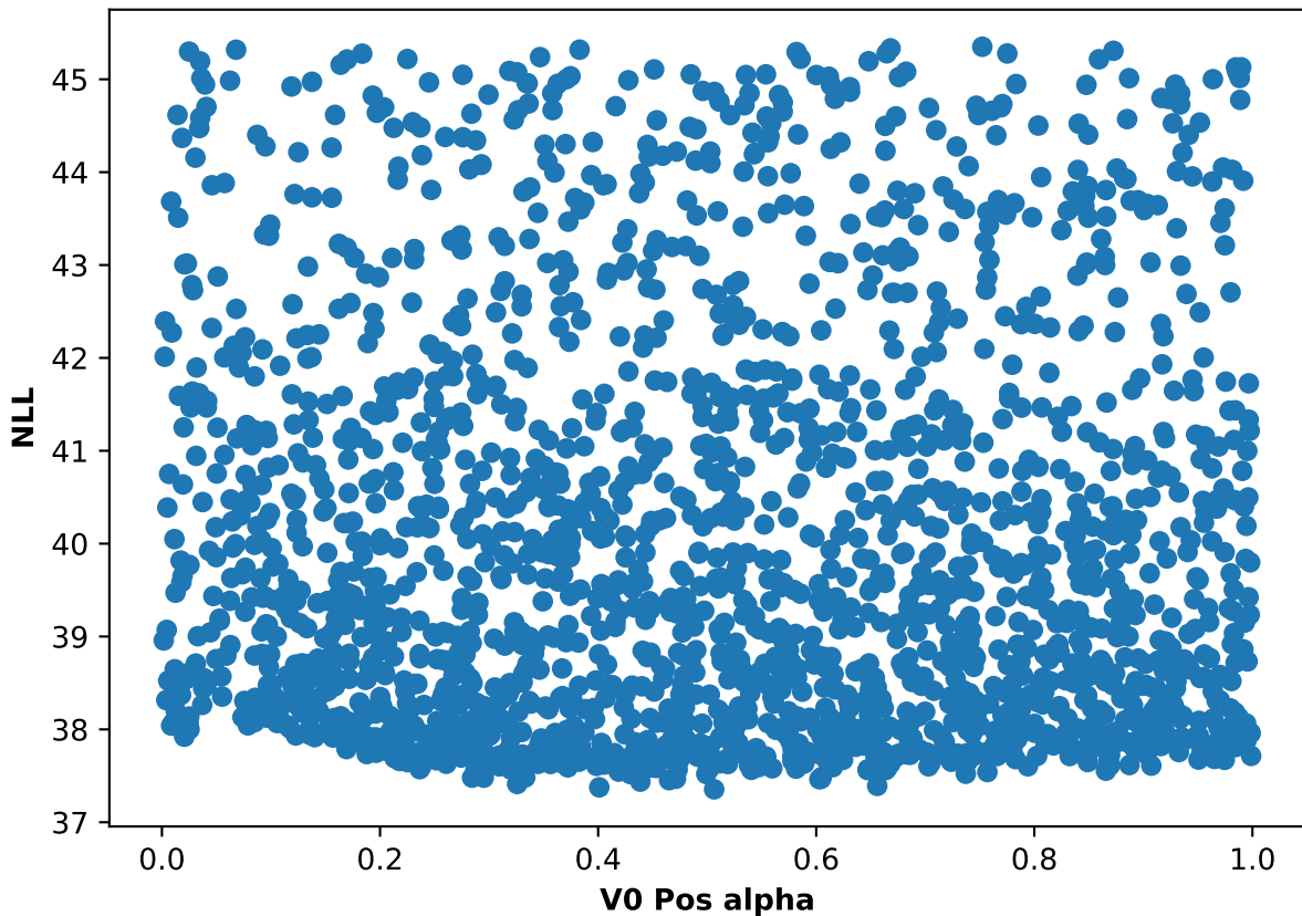
Participant 03, run 2: NLL and V0 Pos alpha scatter plot
