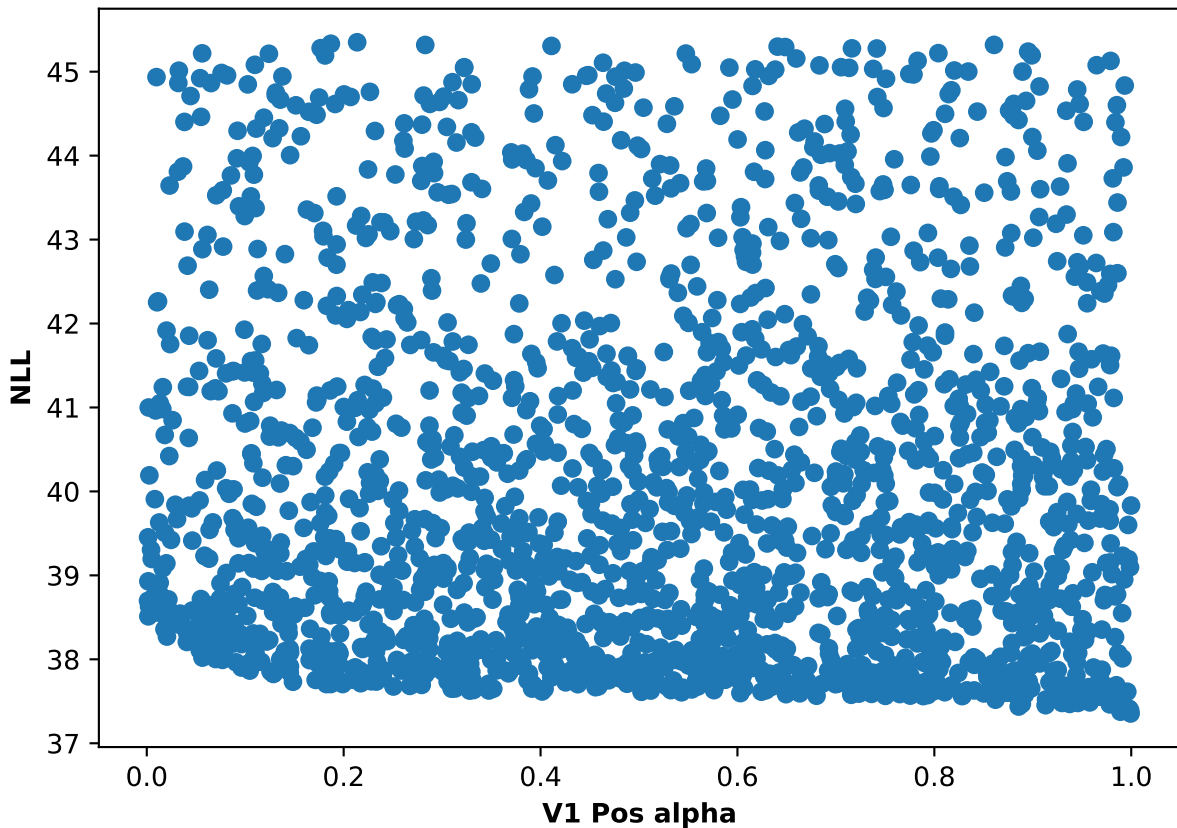
Participant 03, run 2: NLL and V1 Pos alpha scatter plot
