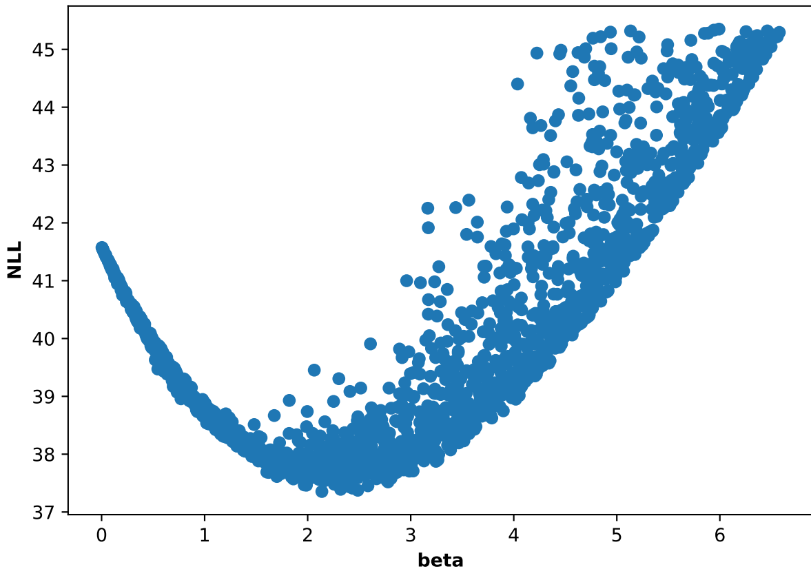
Participant 03, run 2: NLL and beta scatter plot
