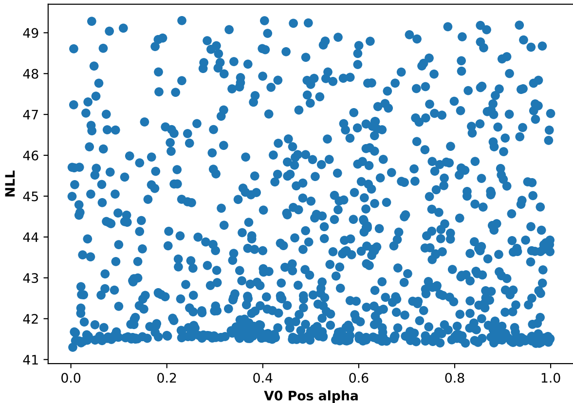
Participant 04, run 2: NLL and V0 Pos alpha scatter plot
