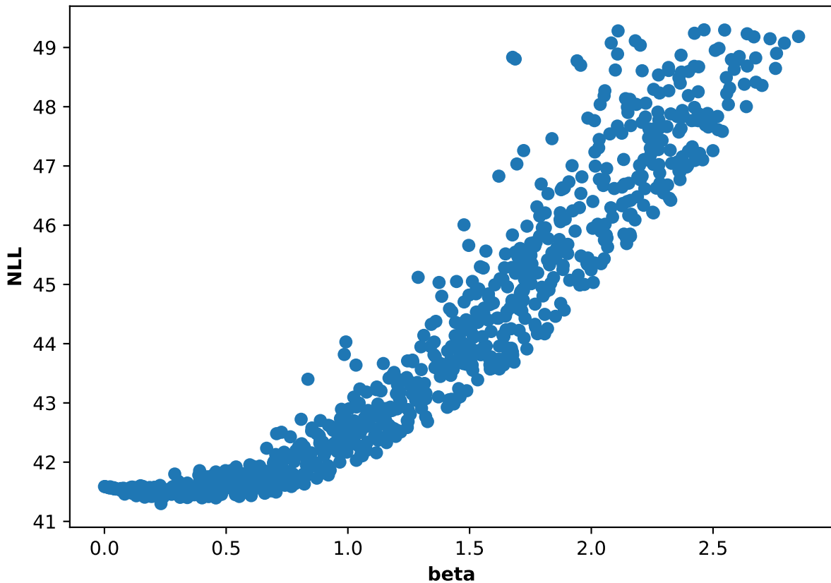
Participant 04, run 2: NLL and beta scatter plot
