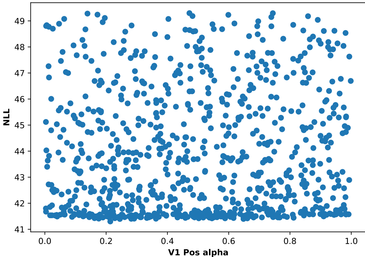
Participant 04, run 2: NLL and V1 Pos alpha scatter plot
