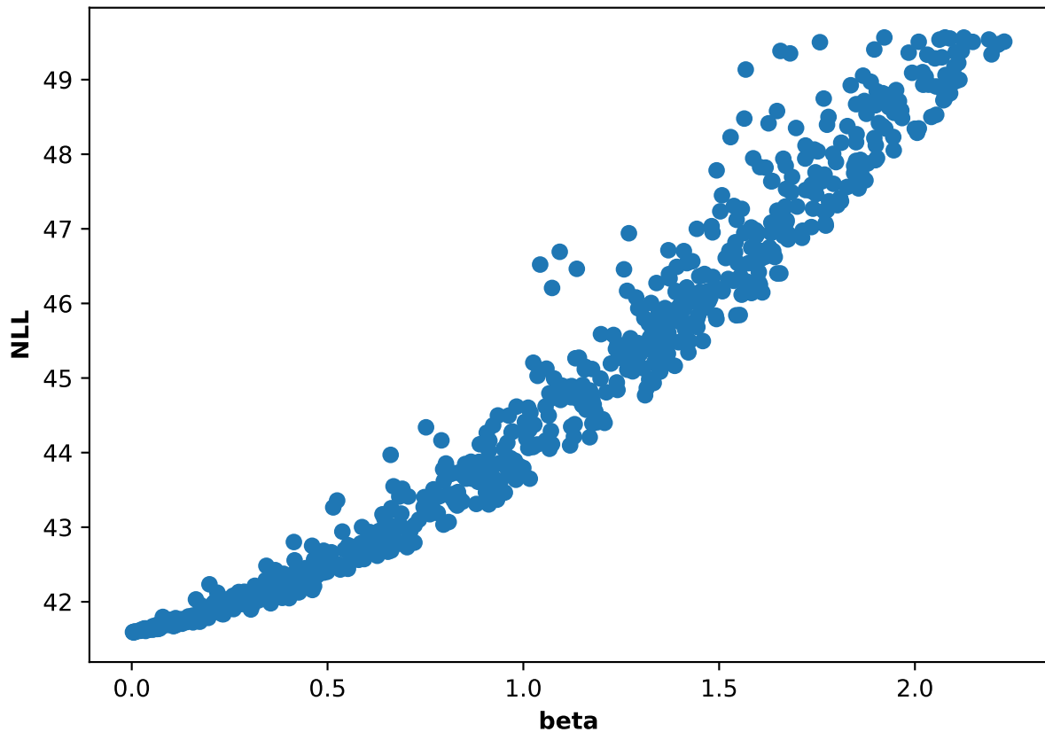
Participant 04, run 3: NLL and beta scatter plot
