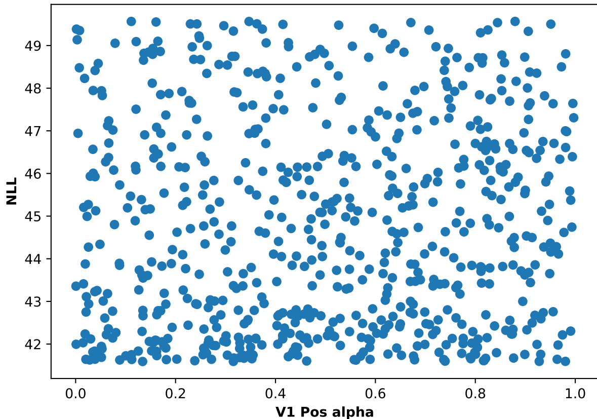
Participant 04, run 3: NLL and V1 Pos alpha scatter plot
