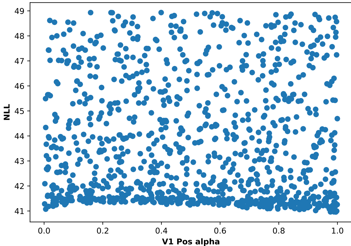
Participant 04, run 4: NLL and V1 Pos alpha scatter plot
