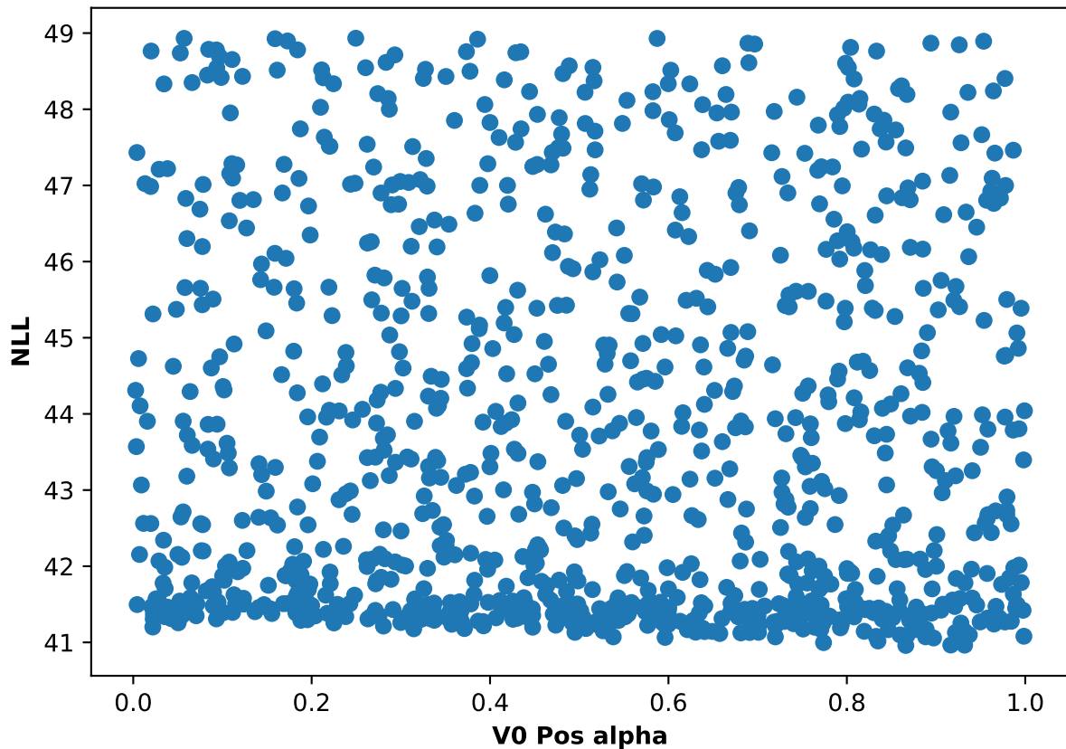
Participant 04, run 4: NLL and V0 Pos alpha scatter plot
