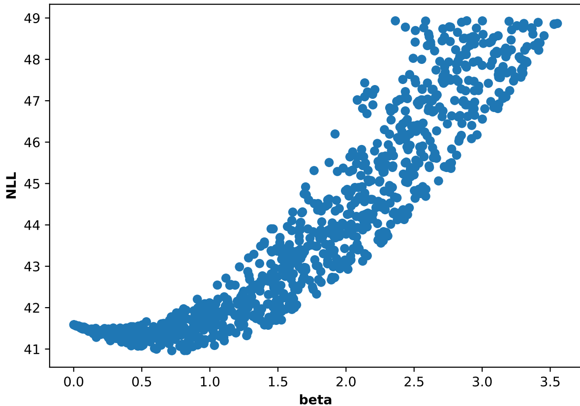
Participant 04, run 4: NLL and beta scatter plot
