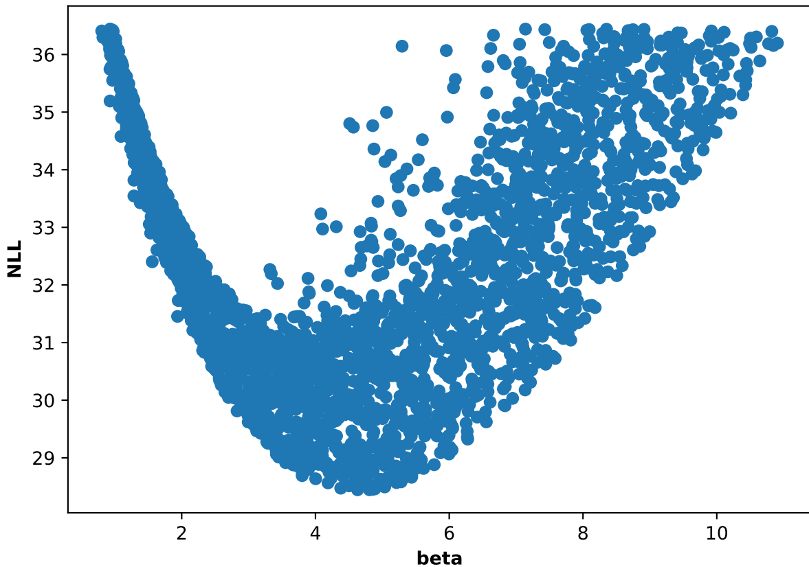
Participant 05, run 3: NLL and beta scatter plot
