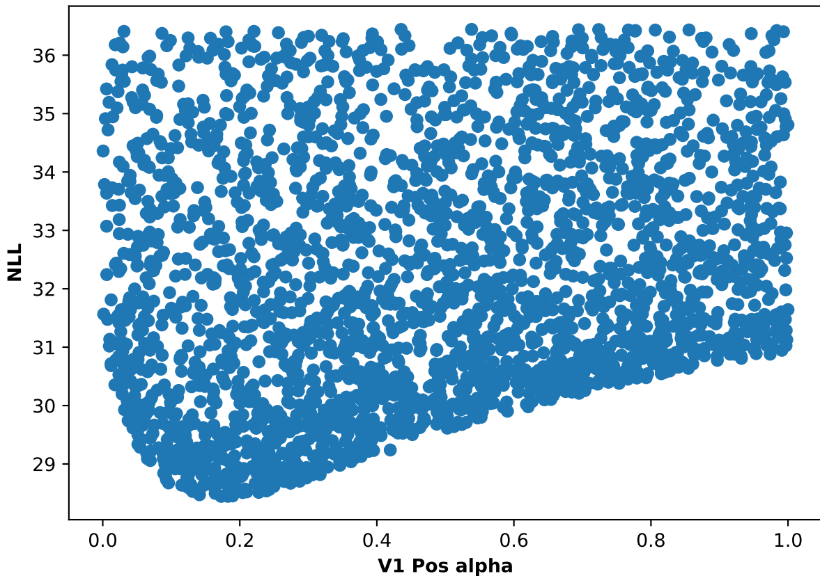
Participant 05, run 3: NLL and V1 Pos alpha scatter plot
