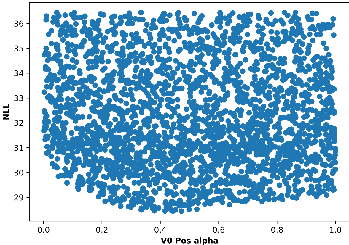
Participant 05, run 3: NLL and V0 Pos alpha scatter plot
