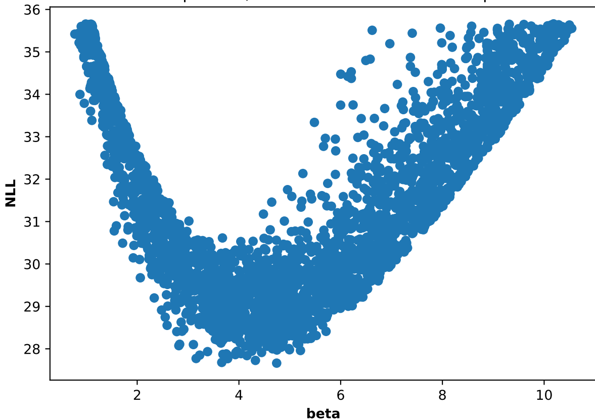
Participant 05, run 4: NLL and beta scatter plot
