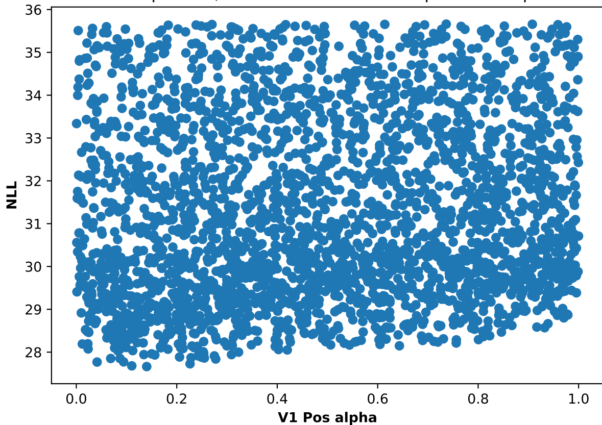
Participant 05, run 4: NLL and V1 Pos alpha scatter plot
