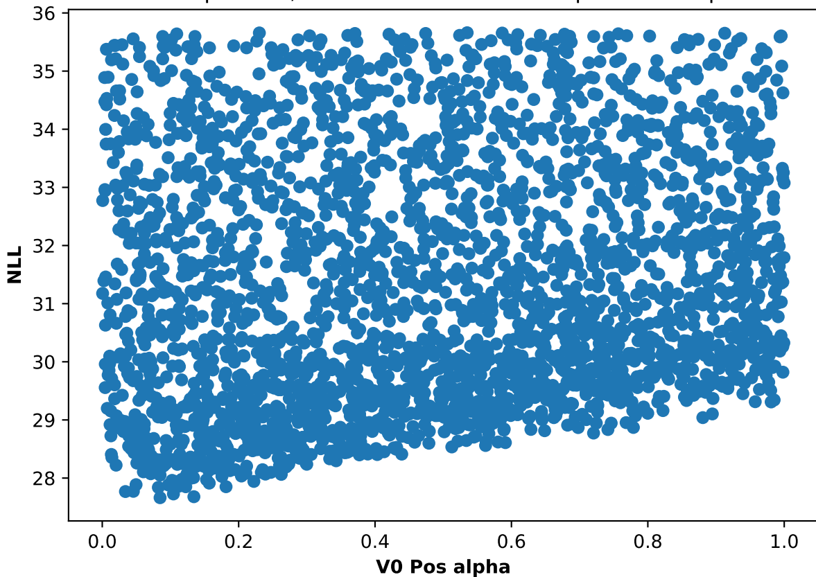
Participant 05, run 4: NLL and V0 Pos alpha scatter plot
