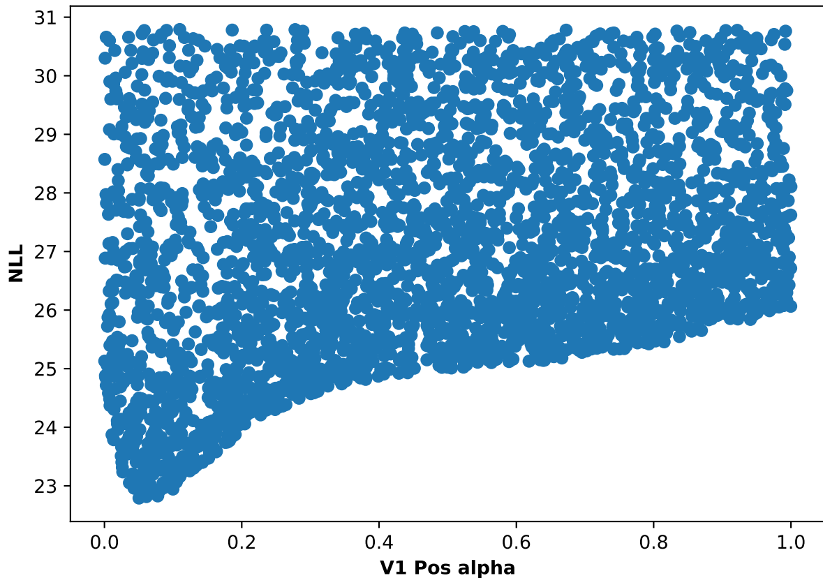
Participant 05, run 5: NLL and V1 Pos alpha scatter plot
