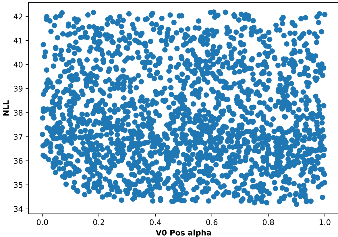
Participant 06, run 3: NLL and V0 Pos alpha scatter plot
