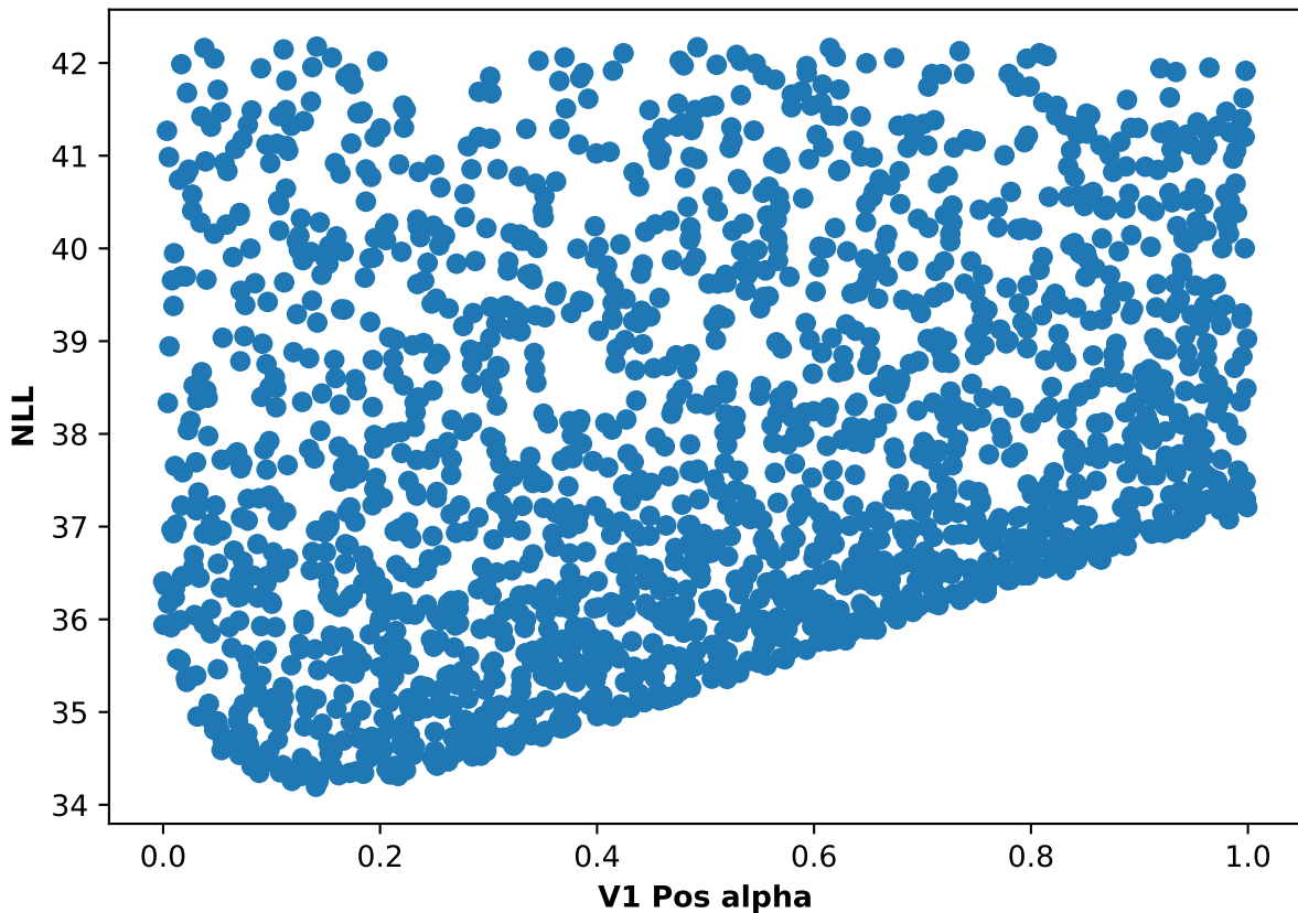
Participant 06, run 3: NLL and V1 Pos alpha scatter plot
