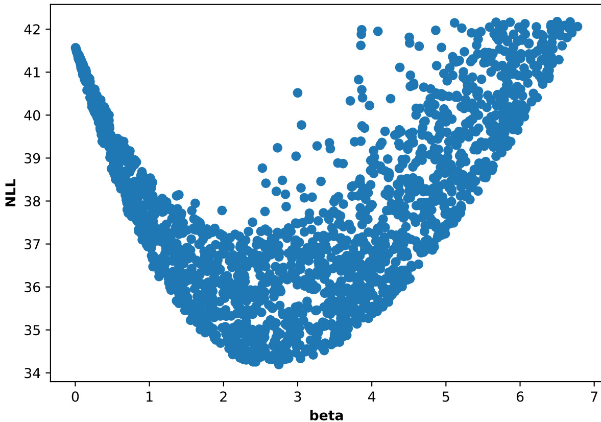
Participant 06, run 3: NLL and beta scatter plot
