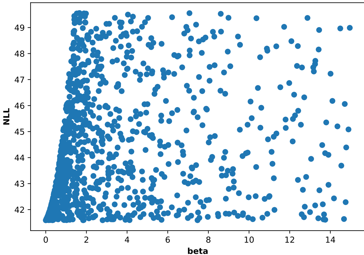
Participant 07, run 2: NLL and beta scatter plot
