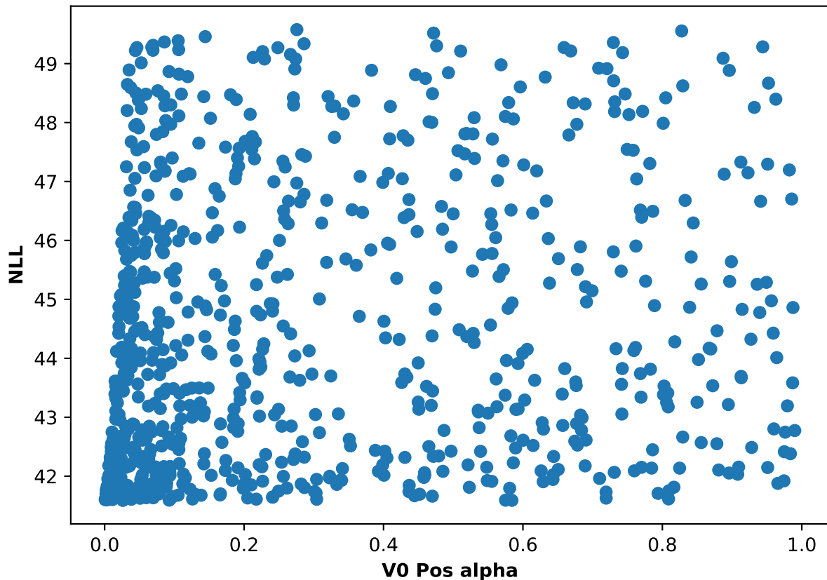
Participant 07, run 3: NLL and V0 Pos alpha scatter plot
