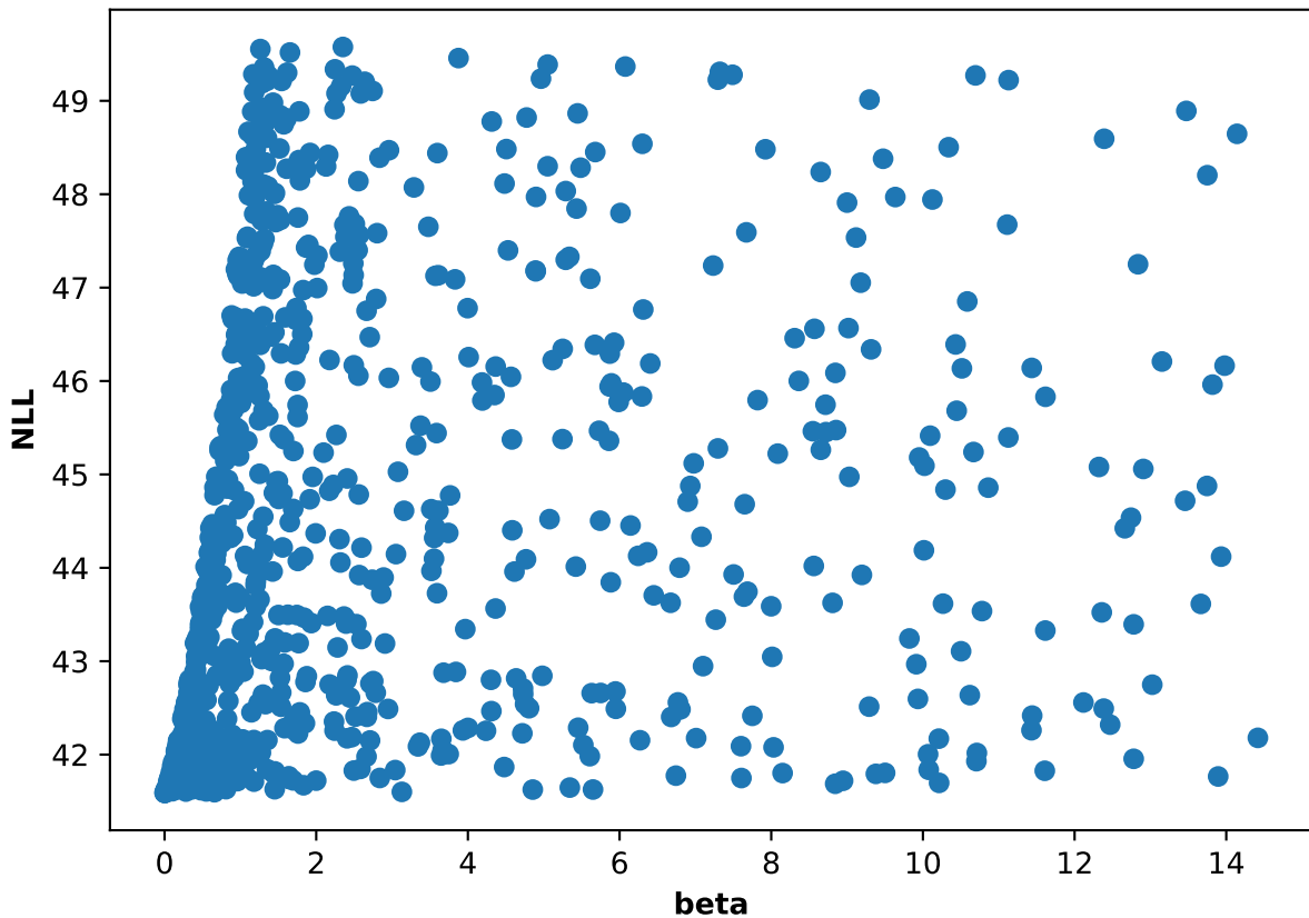
Participant 07, run 3: NLL and beta scatter plot
