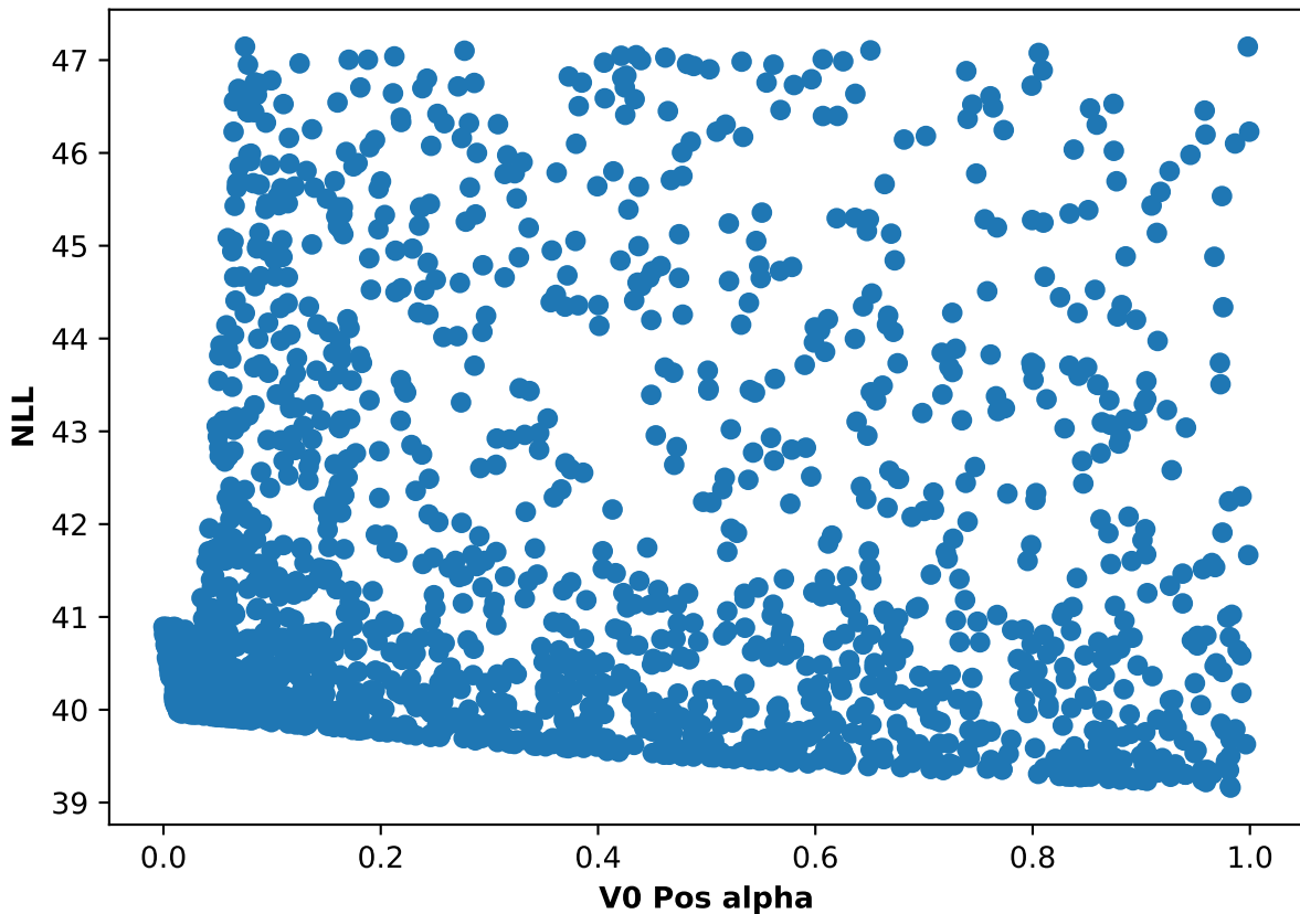
Participant 07, run 4: NLL and V0 Pos alpha scatter plot
