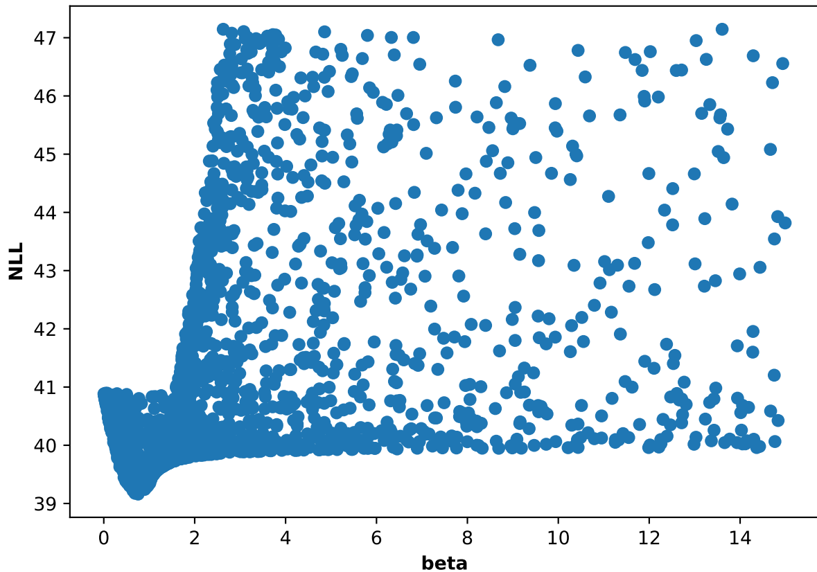
Participant 07, run 4: NLL and beta scatter plot
