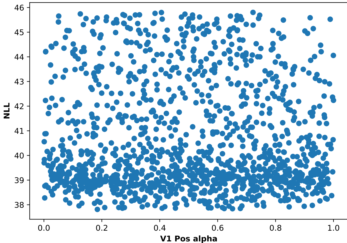
Participant 09, run 1: NLL and V1 Pos alpha scatter plot
