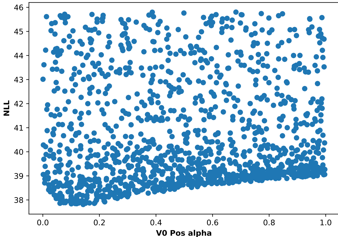
Participant 09, run 1: NLL and V0 Pos alpha scatter plot
