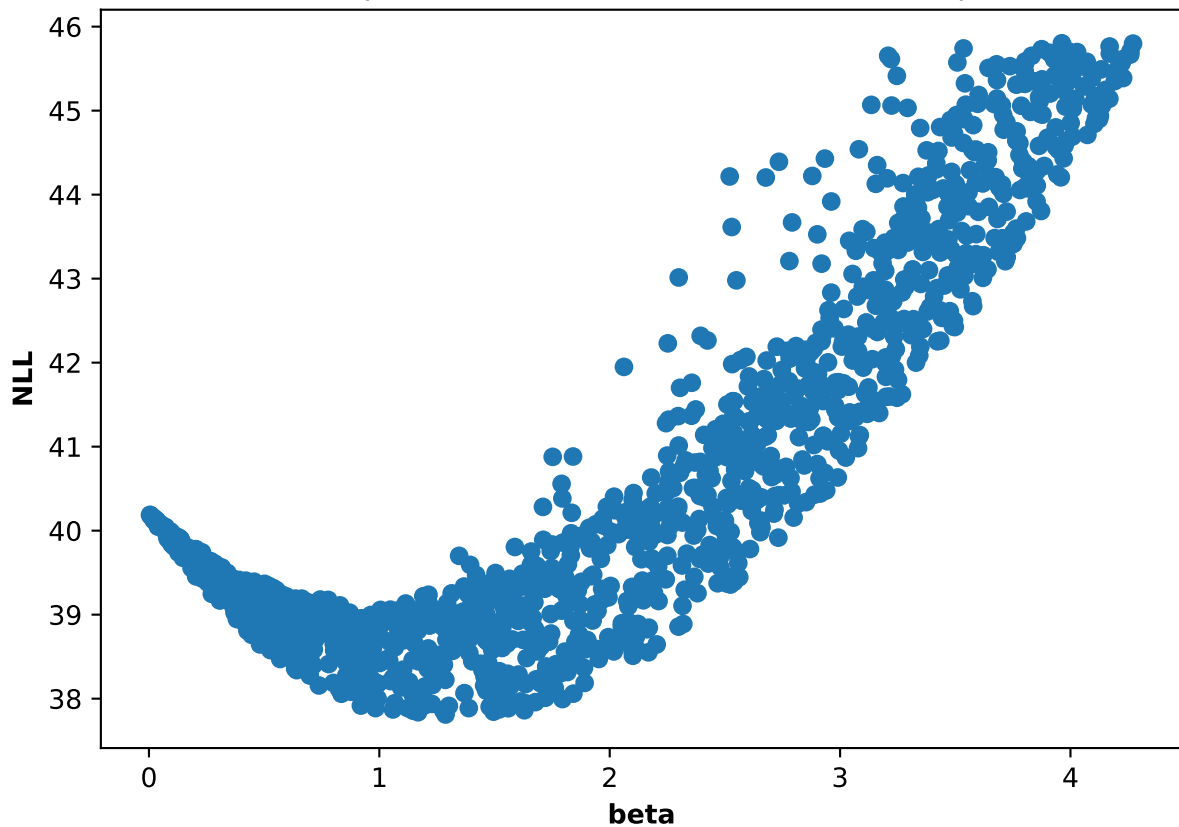
Participant 09, run 1: NLL and beta scatter plot
