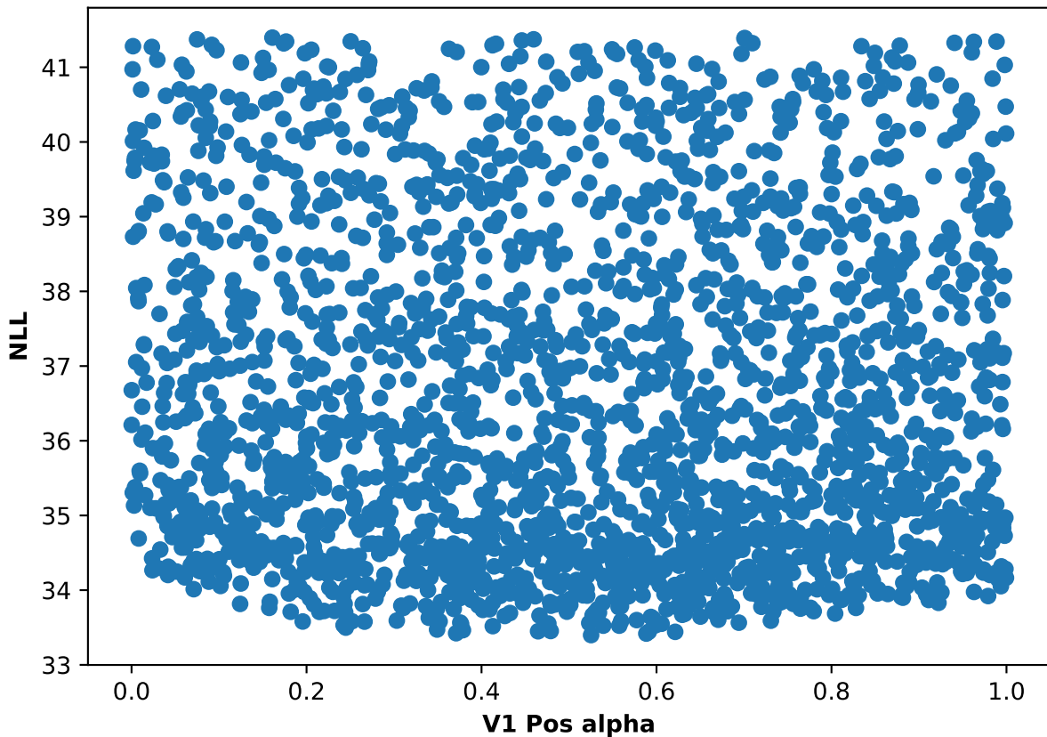
Participant 09, run 3: NLL and V1 Pos alpha scatter plot
