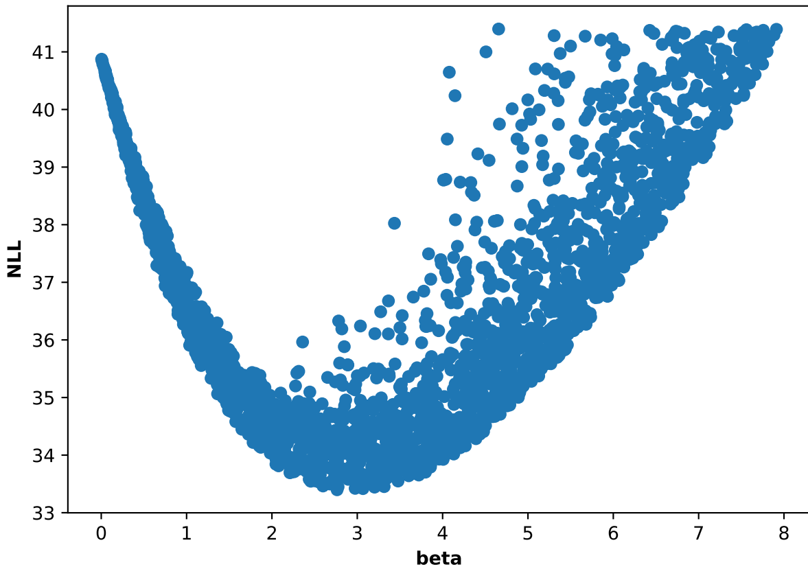
Participant 09, run 3: NLL and beta scatter plot
