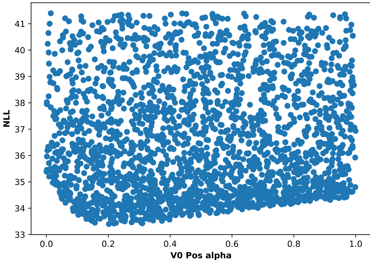
Participant 09, run 3: NLL and V0 Pos alpha scatter plot
