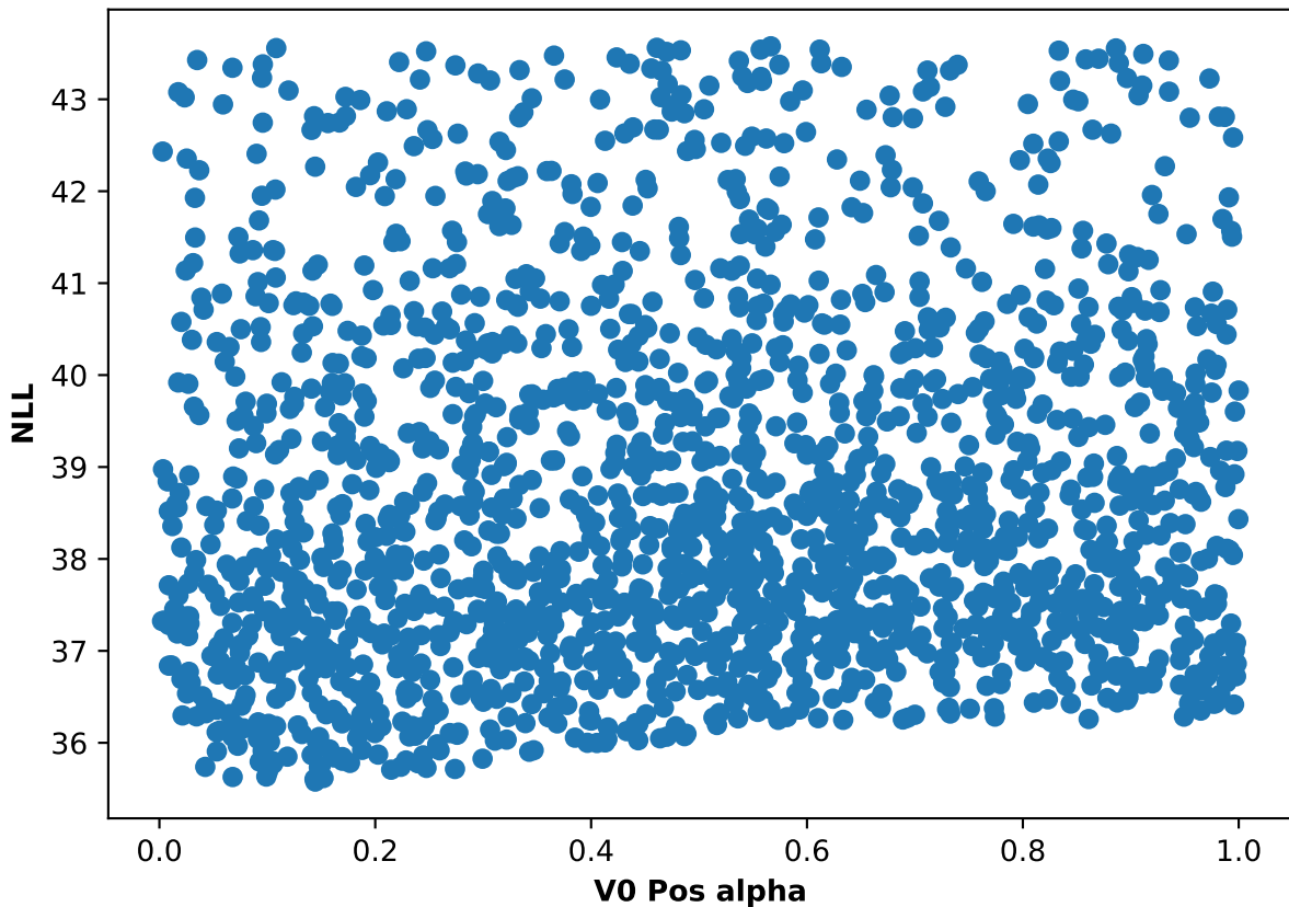
Participant 10, run 1: NLL and V0 Pos alpha scatter plot
