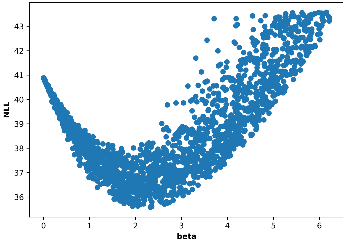
Participant 10, run 1: NLL and beta scatter plot
