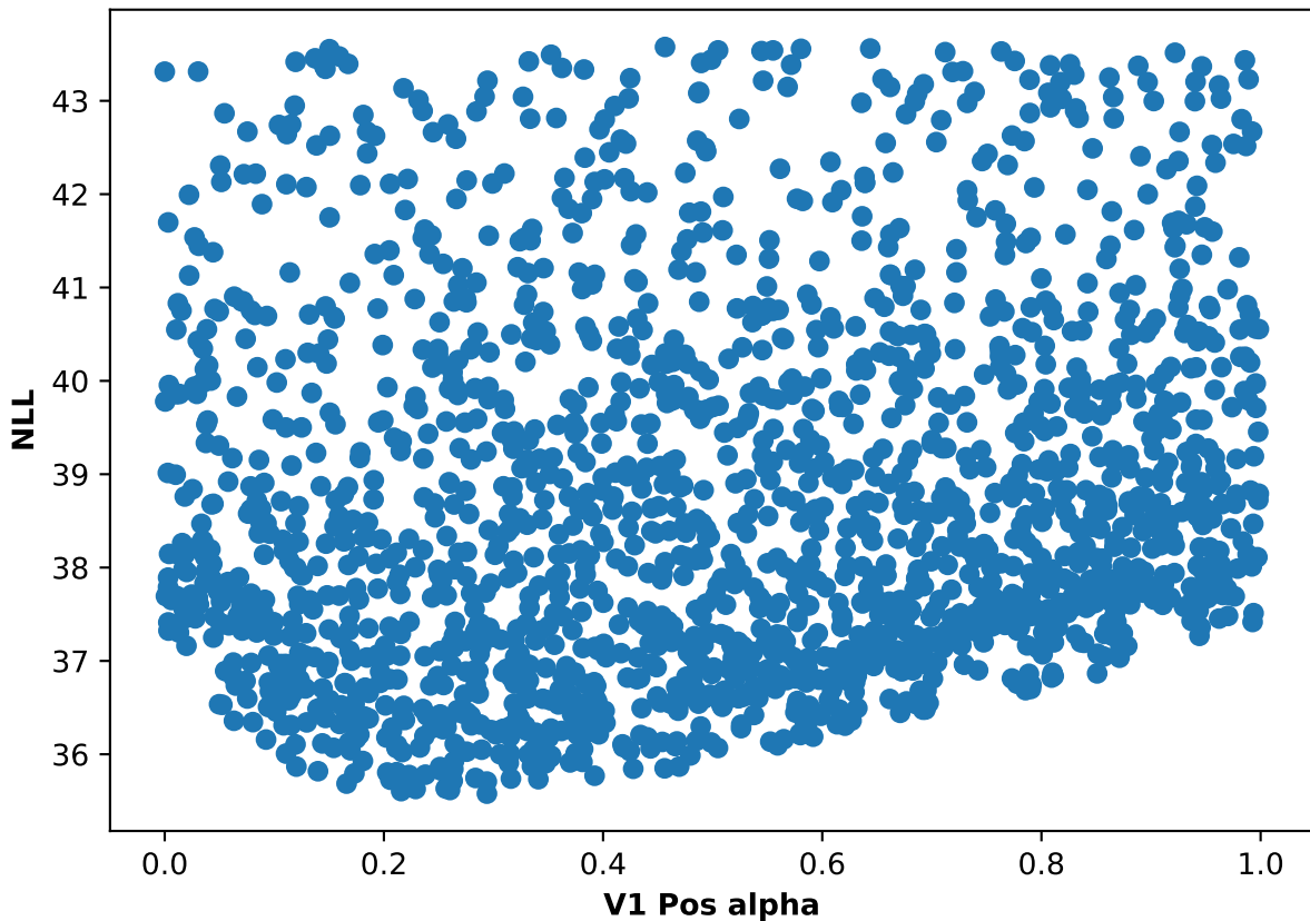
Participant 10, run 1: NLL and V1 Pos alpha scatter plot
