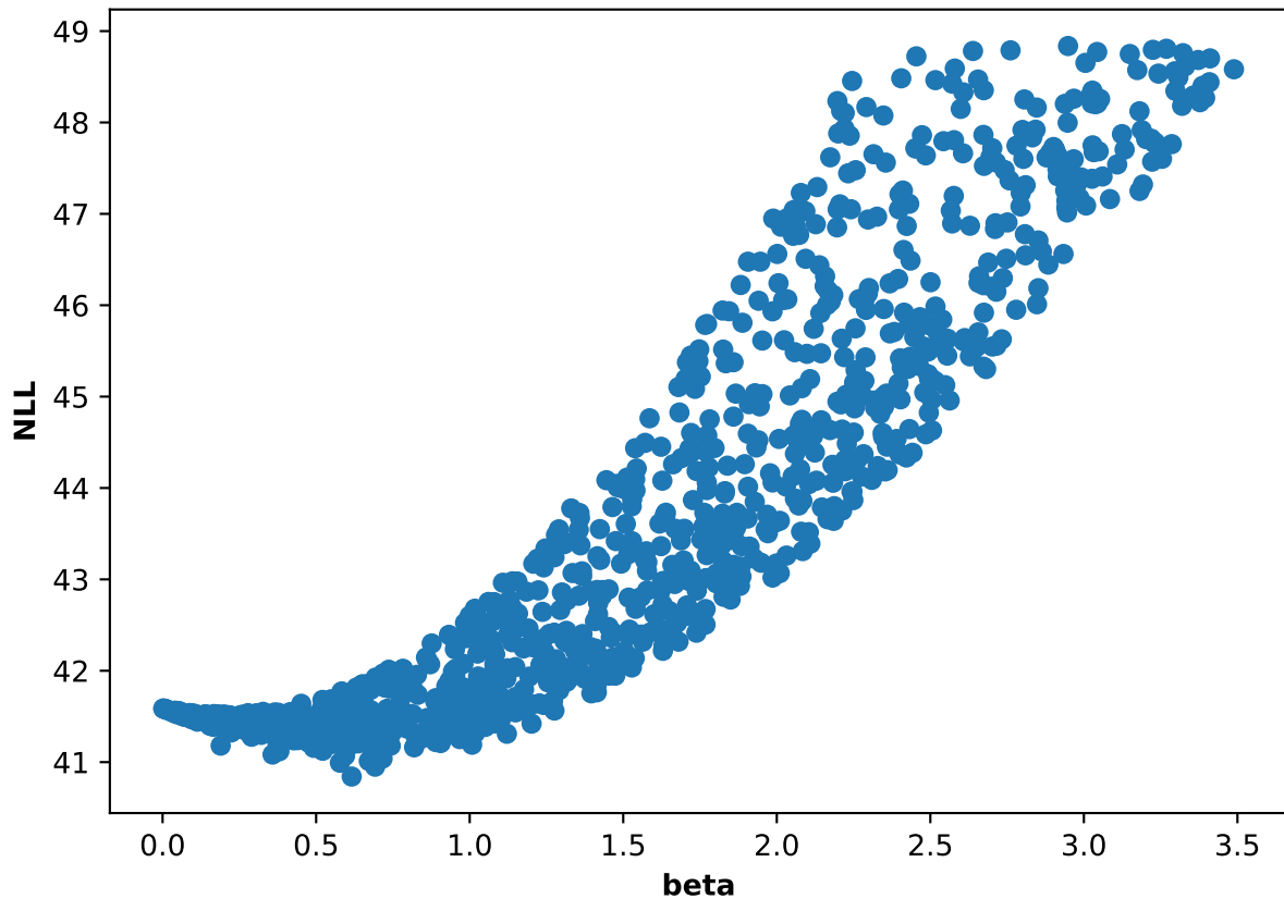
Participant 12, run 2: NLL and beta scatter plot
