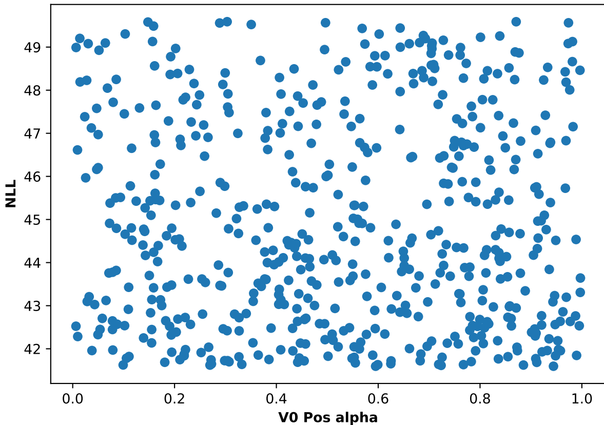
Participant 12, run 3: NLL and V0 Pos alpha scatter plot
