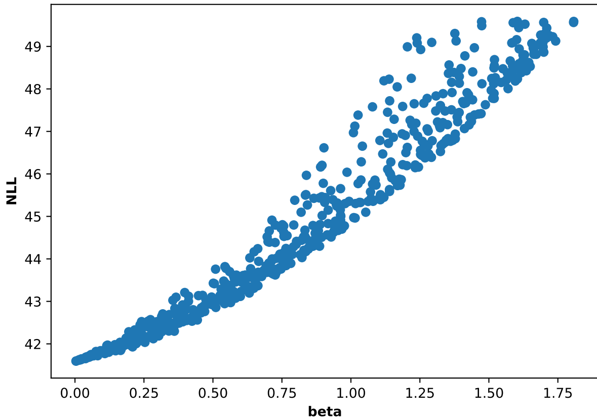
Participant 12, run 3: NLL and beta scatter plot
