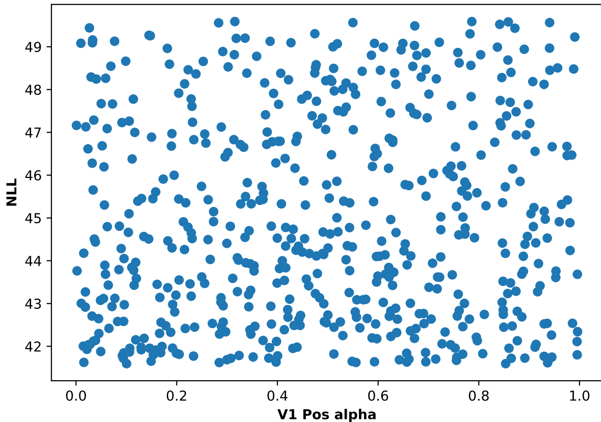
Participant 12, run 3: NLL and V1 Pos alpha scatter plot
