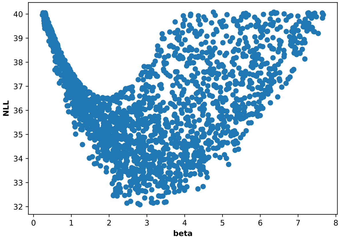
Participant 14, run 3: NLL and beta scatter plot
