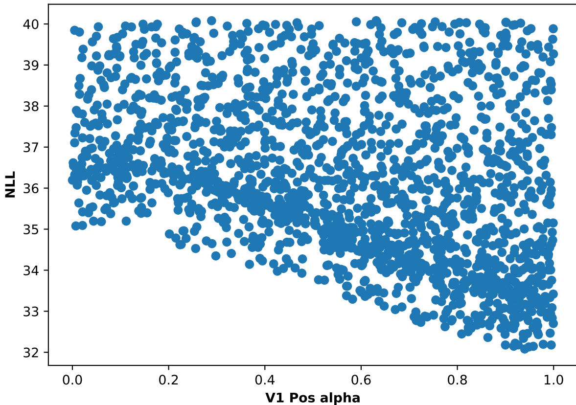
Participant 14, run 3: NLL and V1 Pos alpha scatter plot
