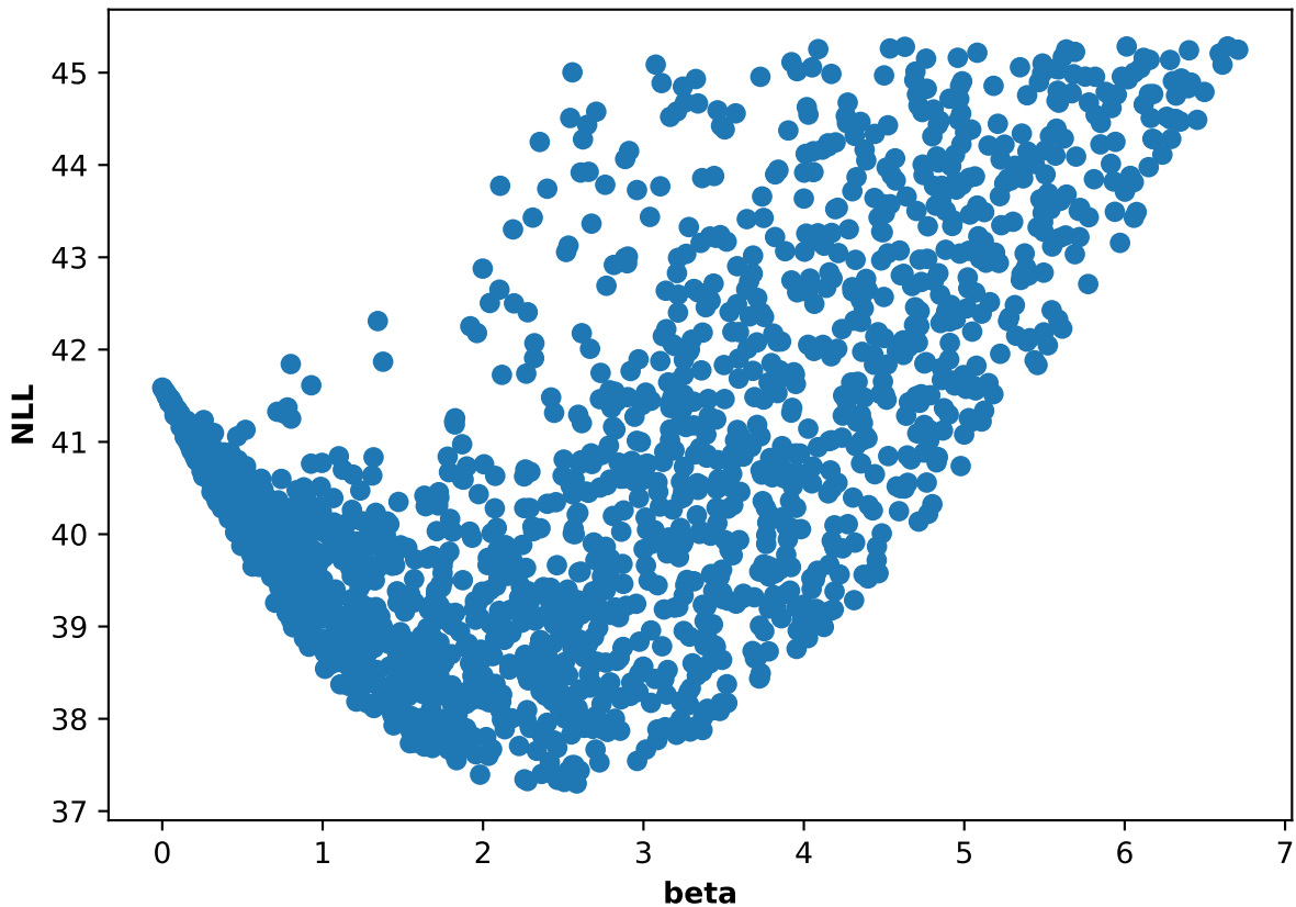
Participant 14, run 4: NLL and beta scatter plot
