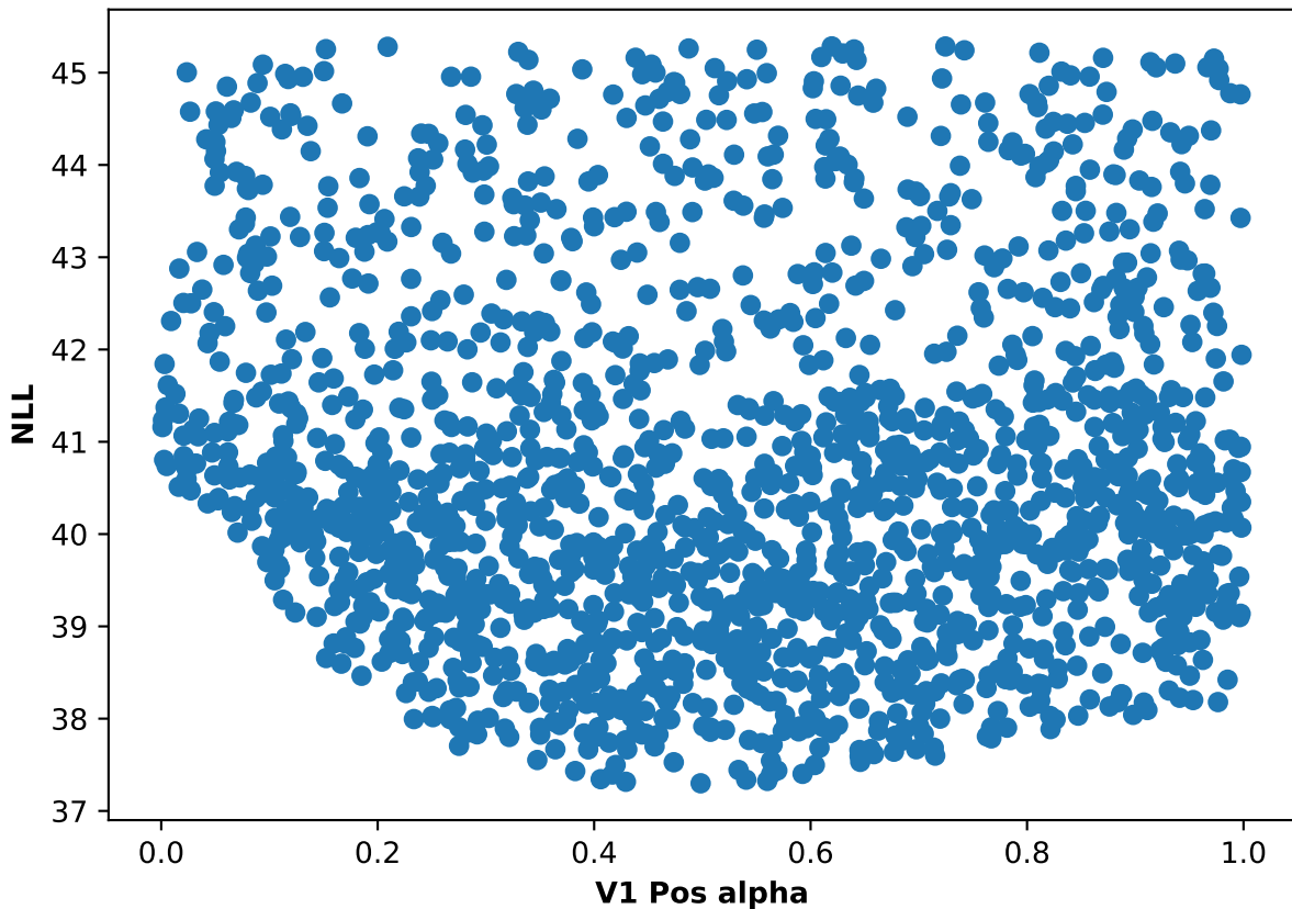
Participant 14, run 4: NLL and V1 Pos alpha scatter plot
