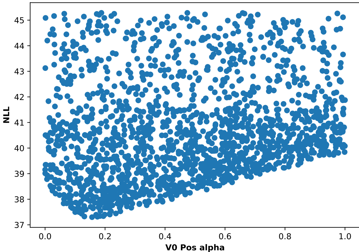
Participant 14, run 4: NLL and V0 Pos alpha scatter plot
