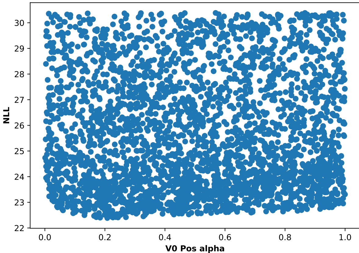
Participant 14, run 5: NLL and V0 Pos alpha scatter plot
