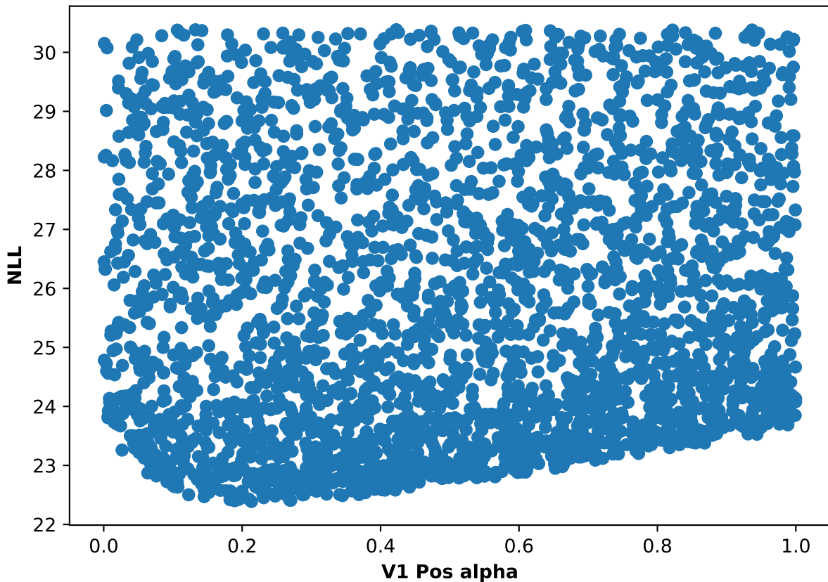
Participant 14, run 5: NLL and V1 Pos alpha scatter plot
