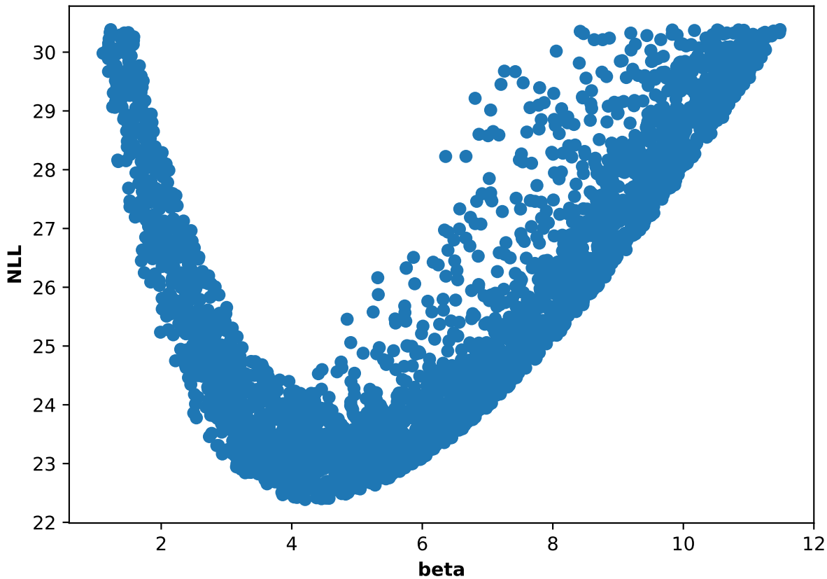
Participant 14, run 5: NLL and beta scatter plot
