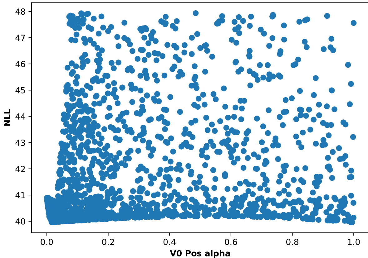
Participant 15, run 1: NLL and V0 Pos alpha scatter plot
