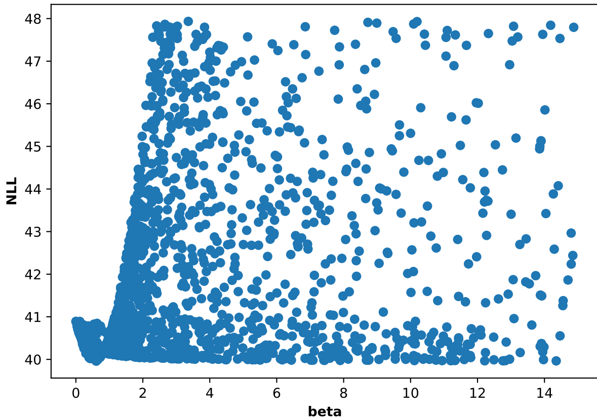
Participant 15, run 1: NLL and beta scatter plot
