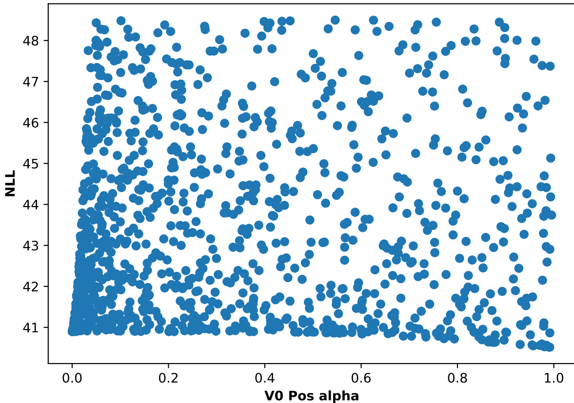
Participant 15, run 5: NLL and V0 Pos alpha scatter plot
