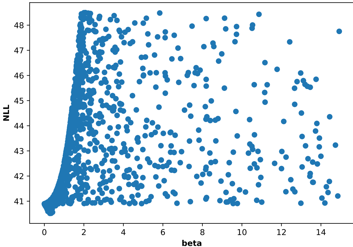
Participant 15, run 5: NLL and beta scatter plot
