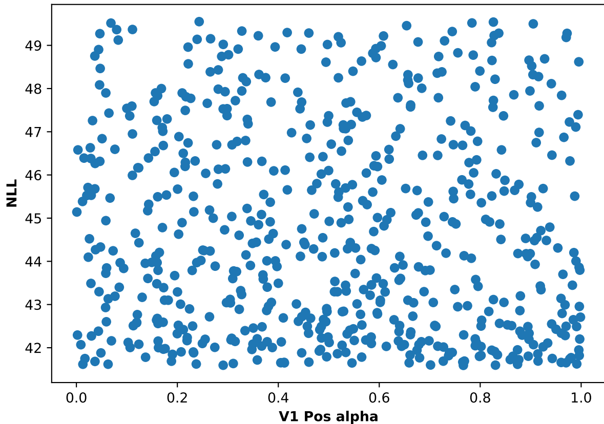
Participant 17, run 2: NLL and V1 Pos alpha scatter plot
