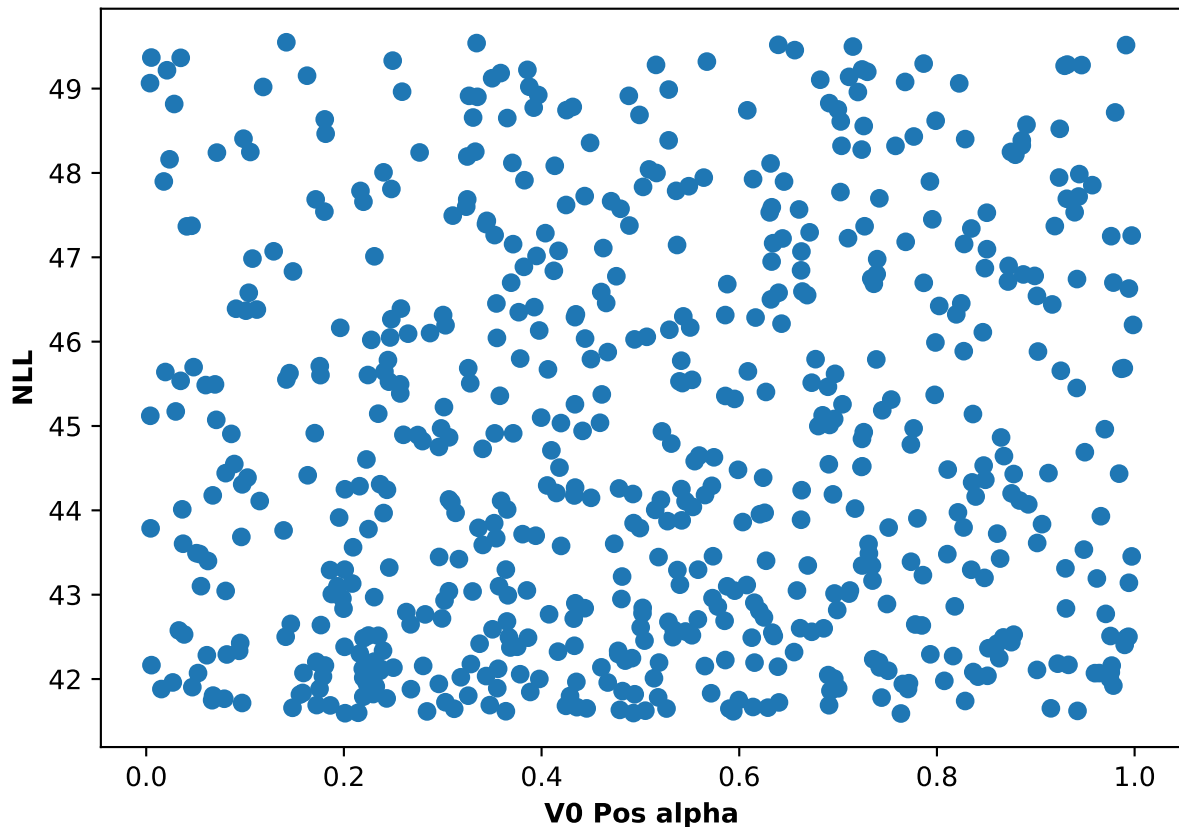
Participant 17, run 2: NLL and V0 Pos alpha scatter plot
