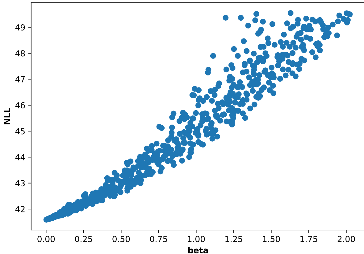
Participant 17, run 2: NLL and beta scatter plot
