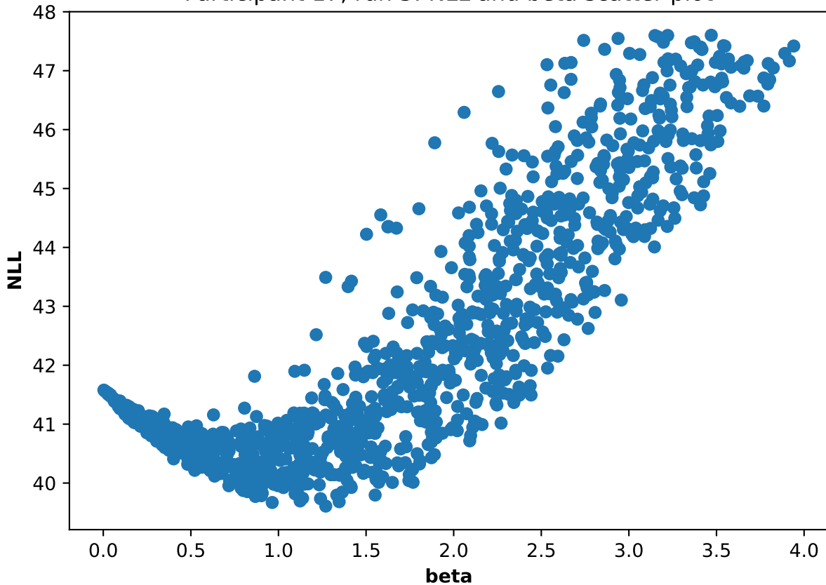
Participant 17, run 5: NLL and beta scatter plot
