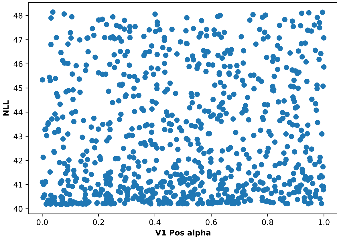
Participant 18, run 1: NLL and V1 Pos alpha scatter plot
