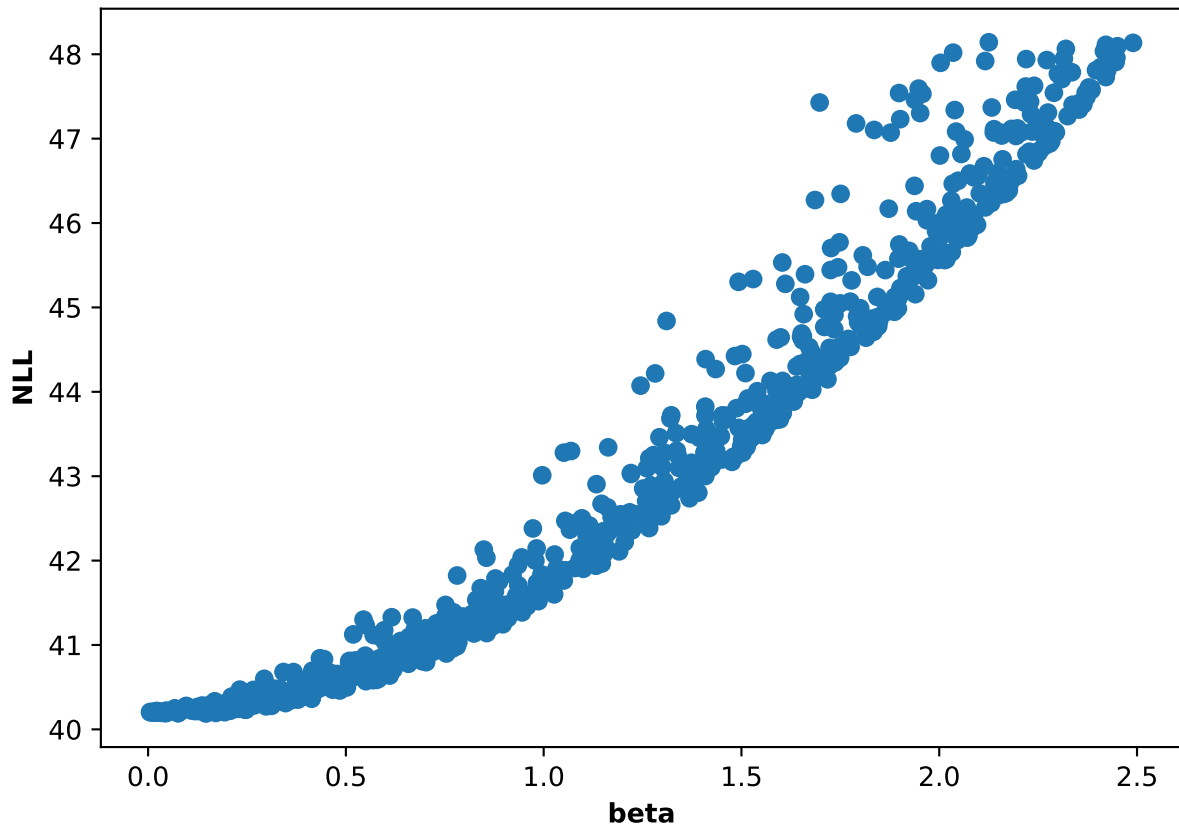
Participant 18, run 1: NLL and beta scatter plot
