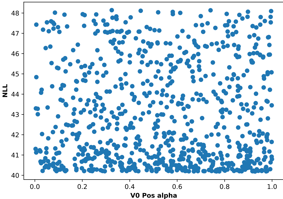
Participant 18, run 1: NLL and V0 Pos alpha scatter plot
