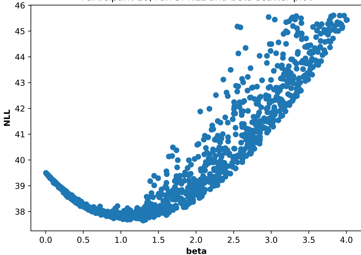
Participant 18, run 3: NLL and beta scatter plot
