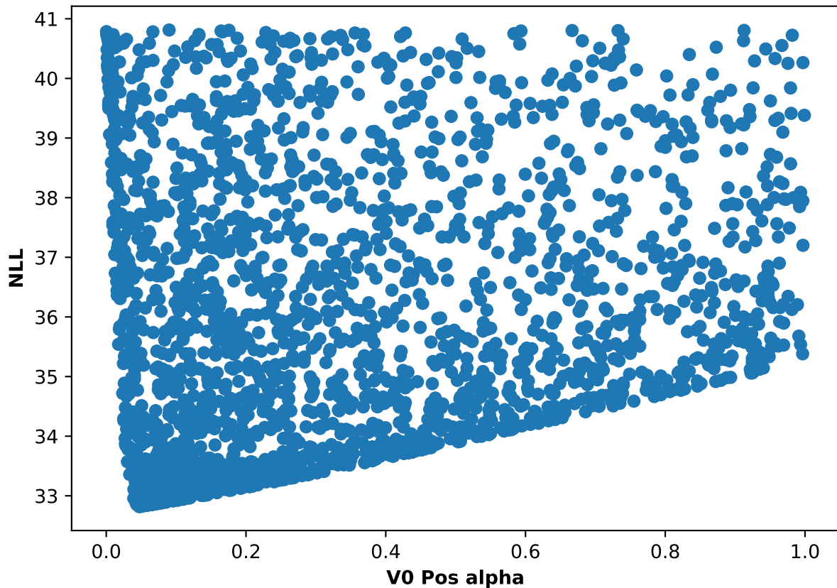
Participant 20, run 3: NLL and V0 Pos alpha scatter plot
