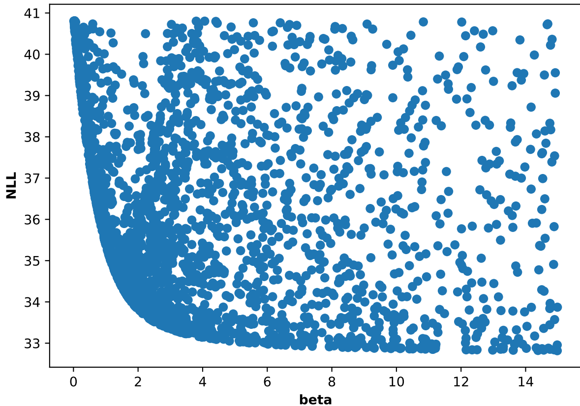
Participant 20, run 3: NLL and beta scatter plot
