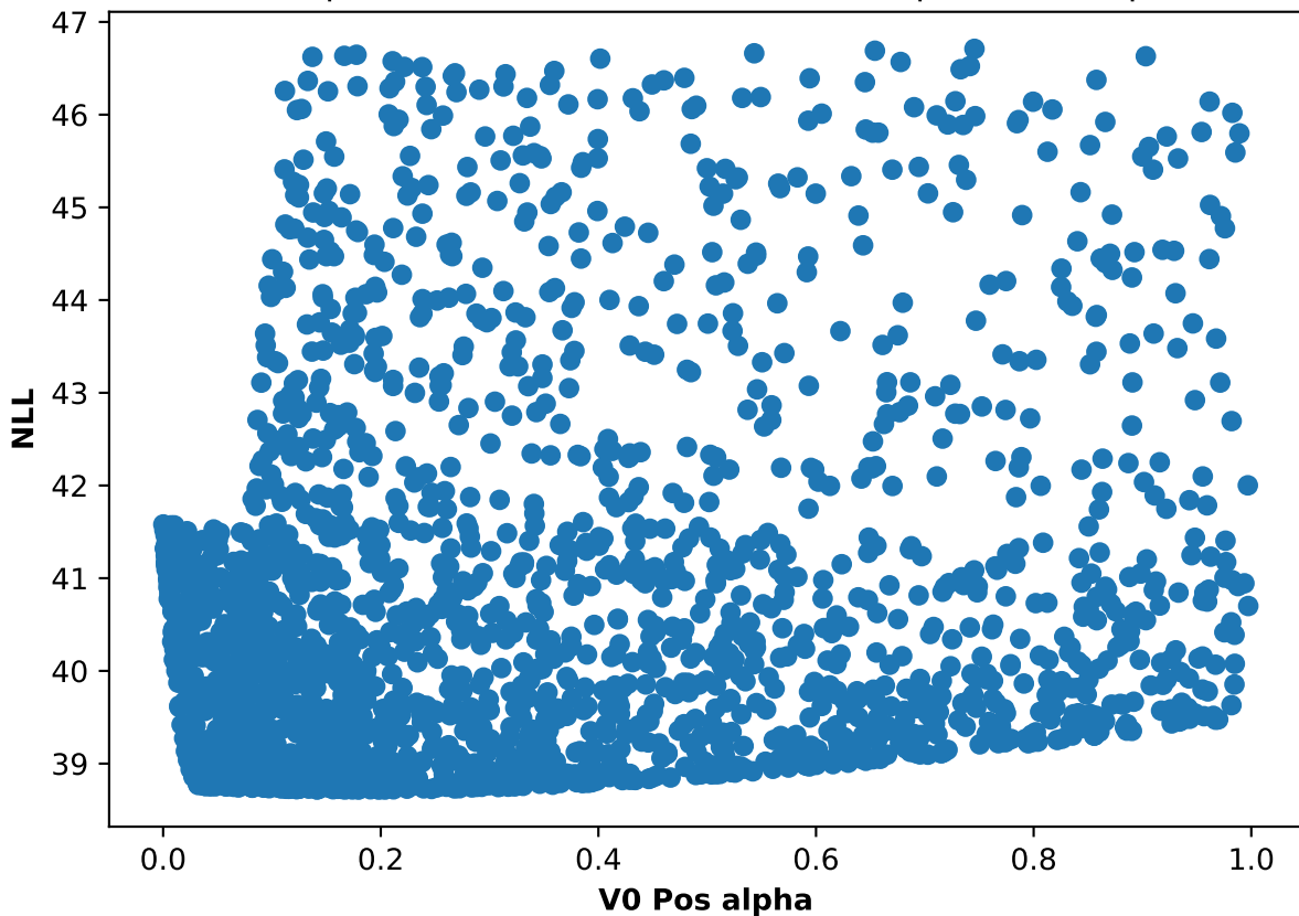
Participant 20, run 4: NLL and V0 Pos alpha scatter plot
