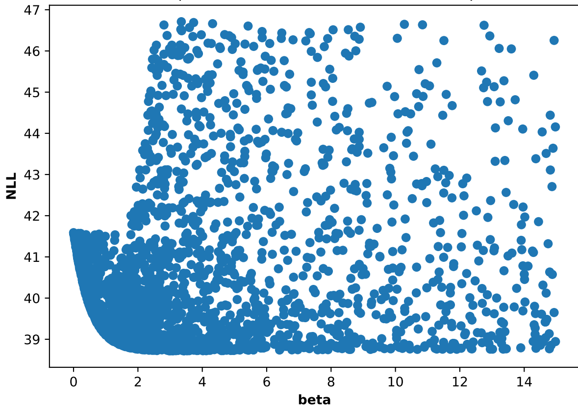
Participant 20, run 4: NLL and beta scatter plot
