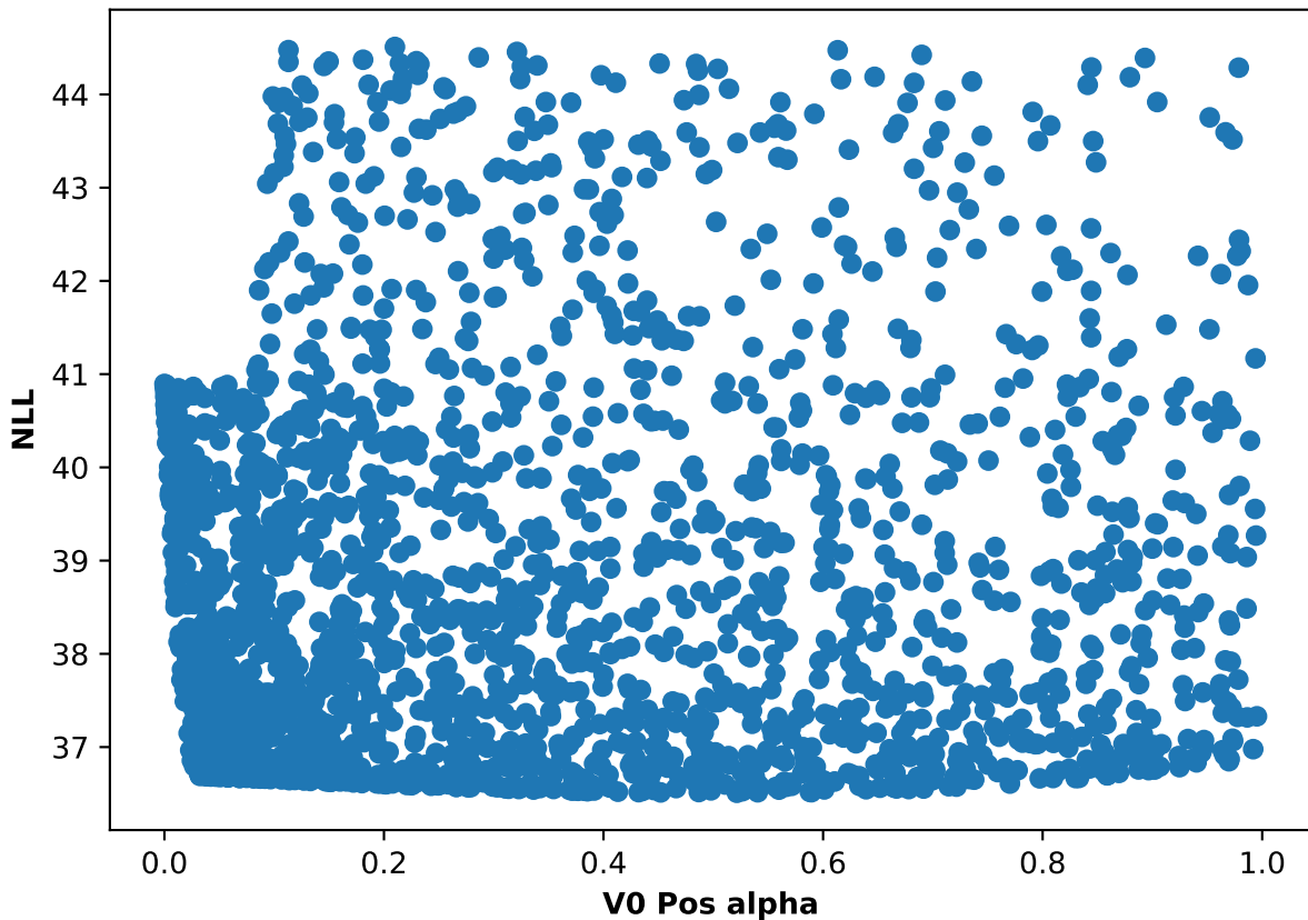
Participant 20, run 5: NLL and V0 Pos alpha scatter plot
