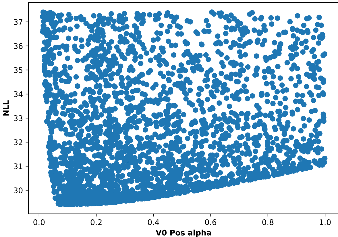
Participant 21, run 3: NLL and V0 Pos alpha scatter plot
