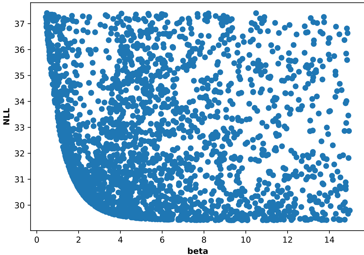
Participant 21, run 3: NLL and beta scatter plot
