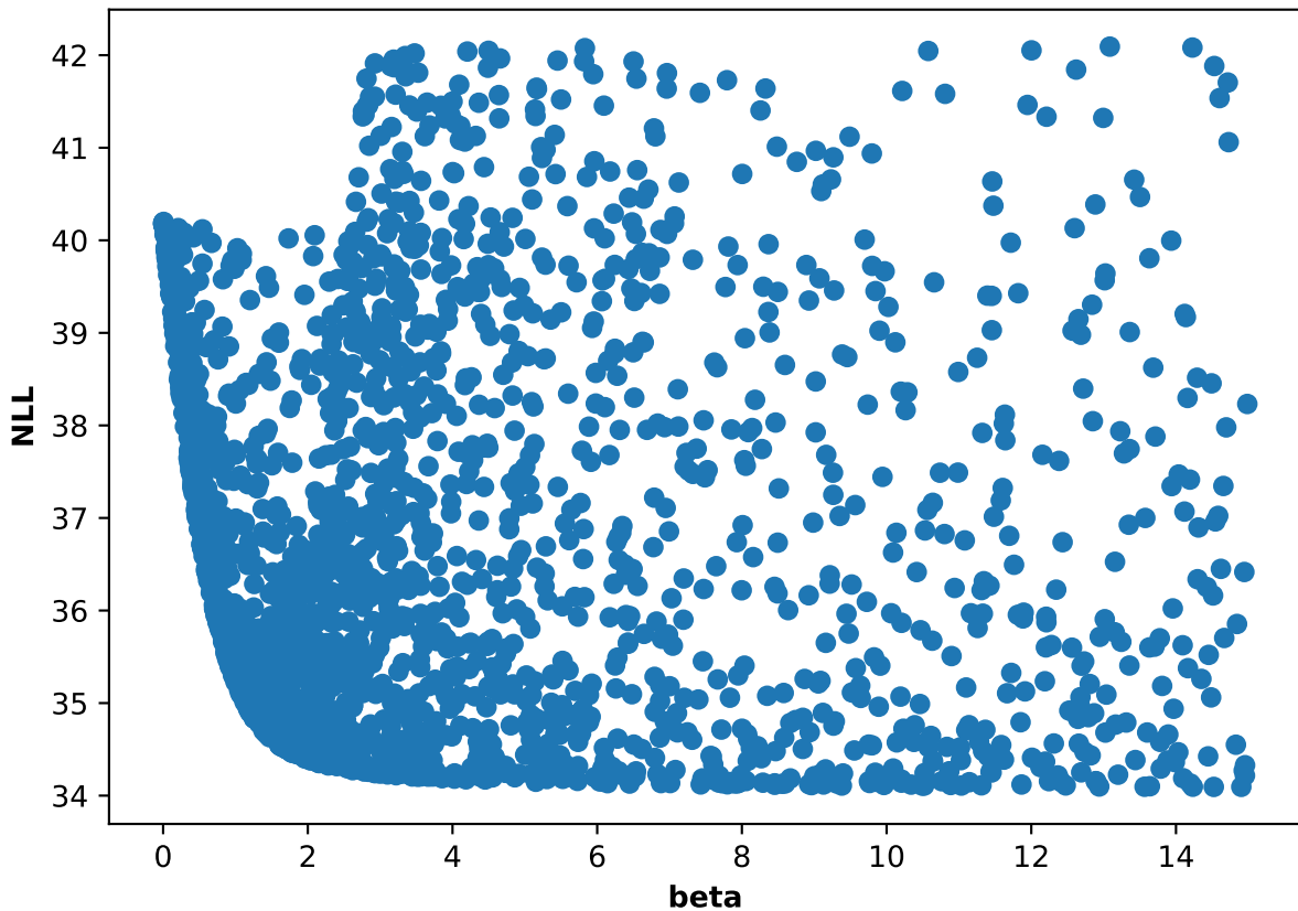
Participant 21, run 5: NLL and beta scatter plot
