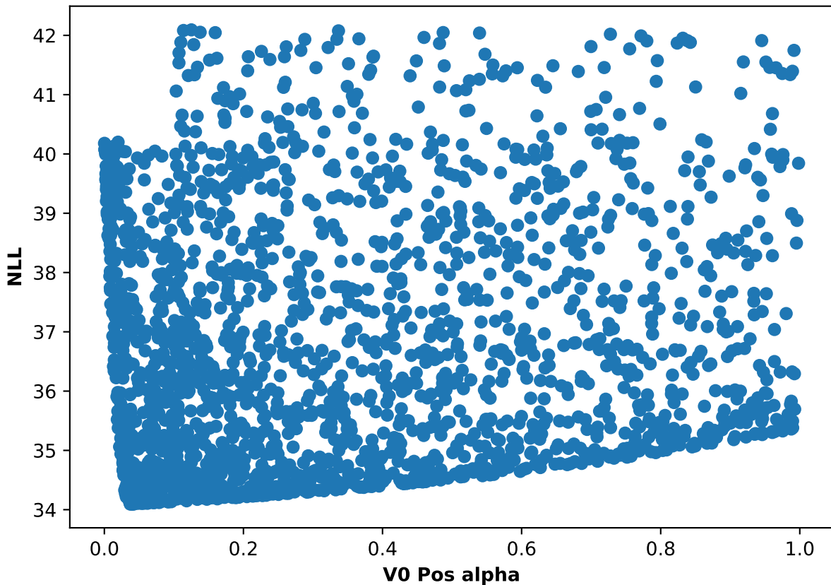
Participant 21, run 5: NLL and V0 Pos alpha scatter plot
