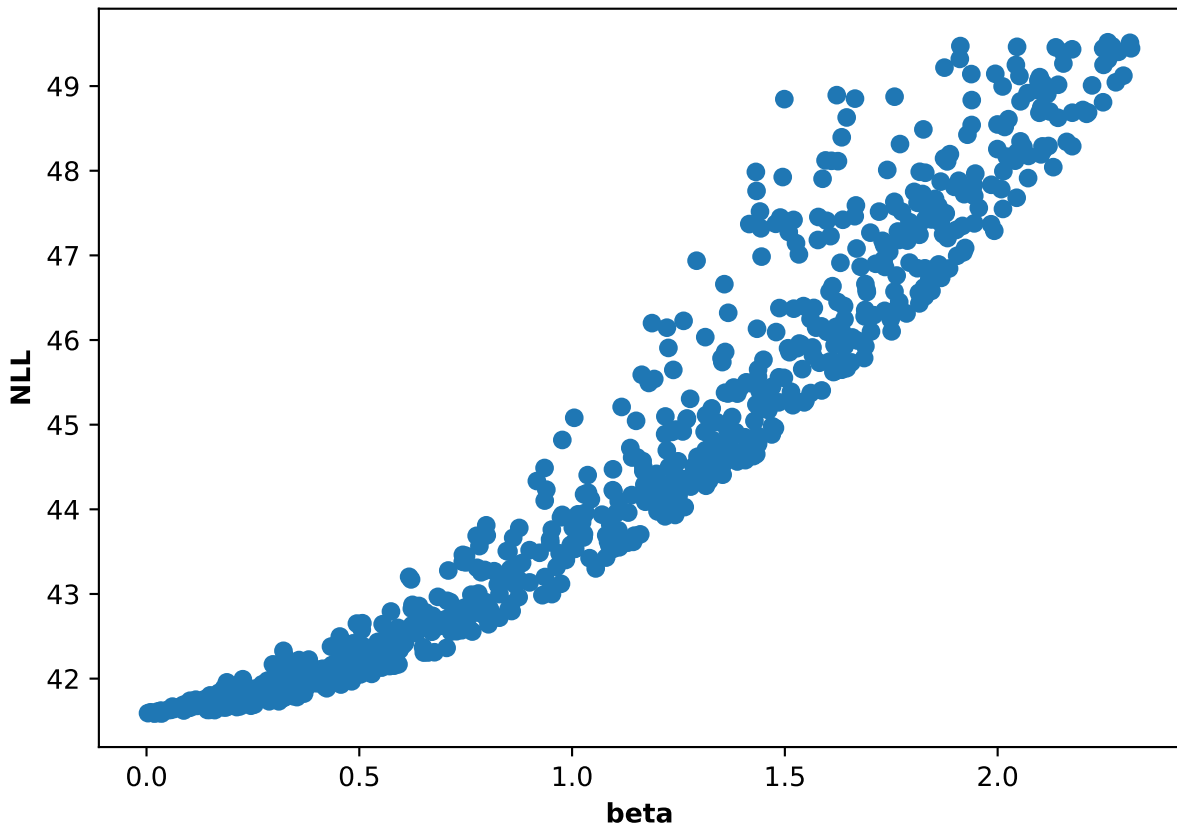
Participant 22, run 1: NLL and beta scatter plot
