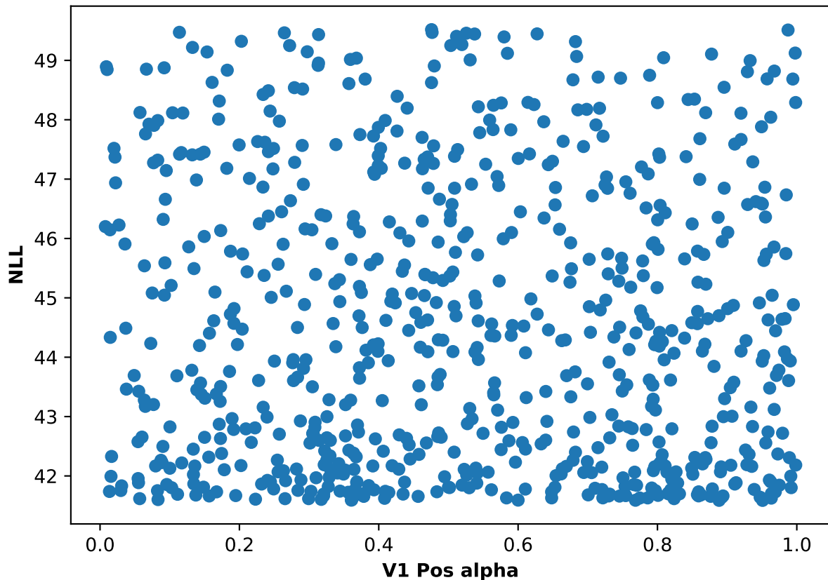
Participant 22, run 1: NLL and V1 Pos alpha scatter plot
