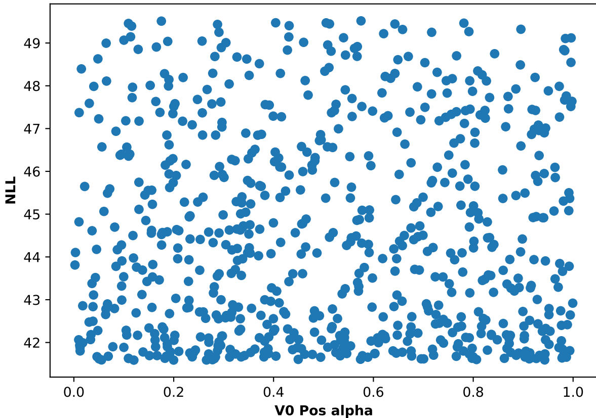
Participant 22, run 1: NLL and V0 Pos alpha scatter plot
