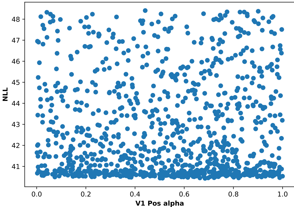
Participant 22, run 3: NLL and V1 Pos alpha scatter plot
