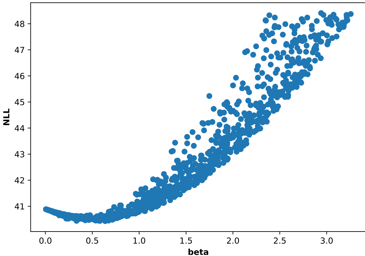
Participant 22, run 3: NLL and beta scatter plot
