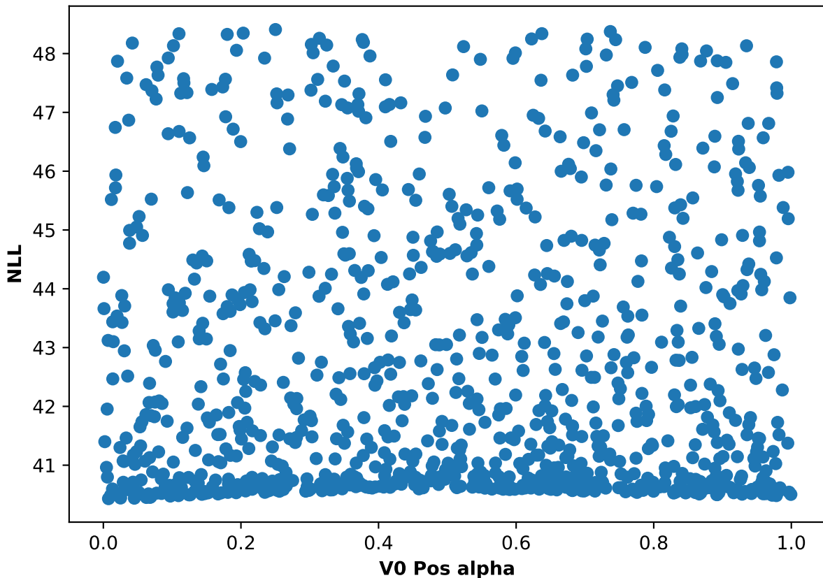
Participant 22, run 3: NLL and V0 Pos alpha scatter plot
