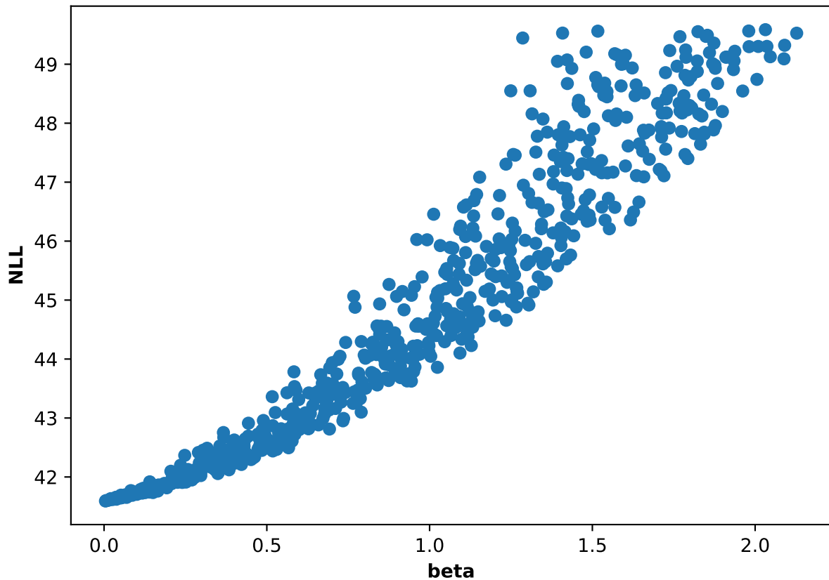
Participant 23, run 5: NLL and beta scatter plot
