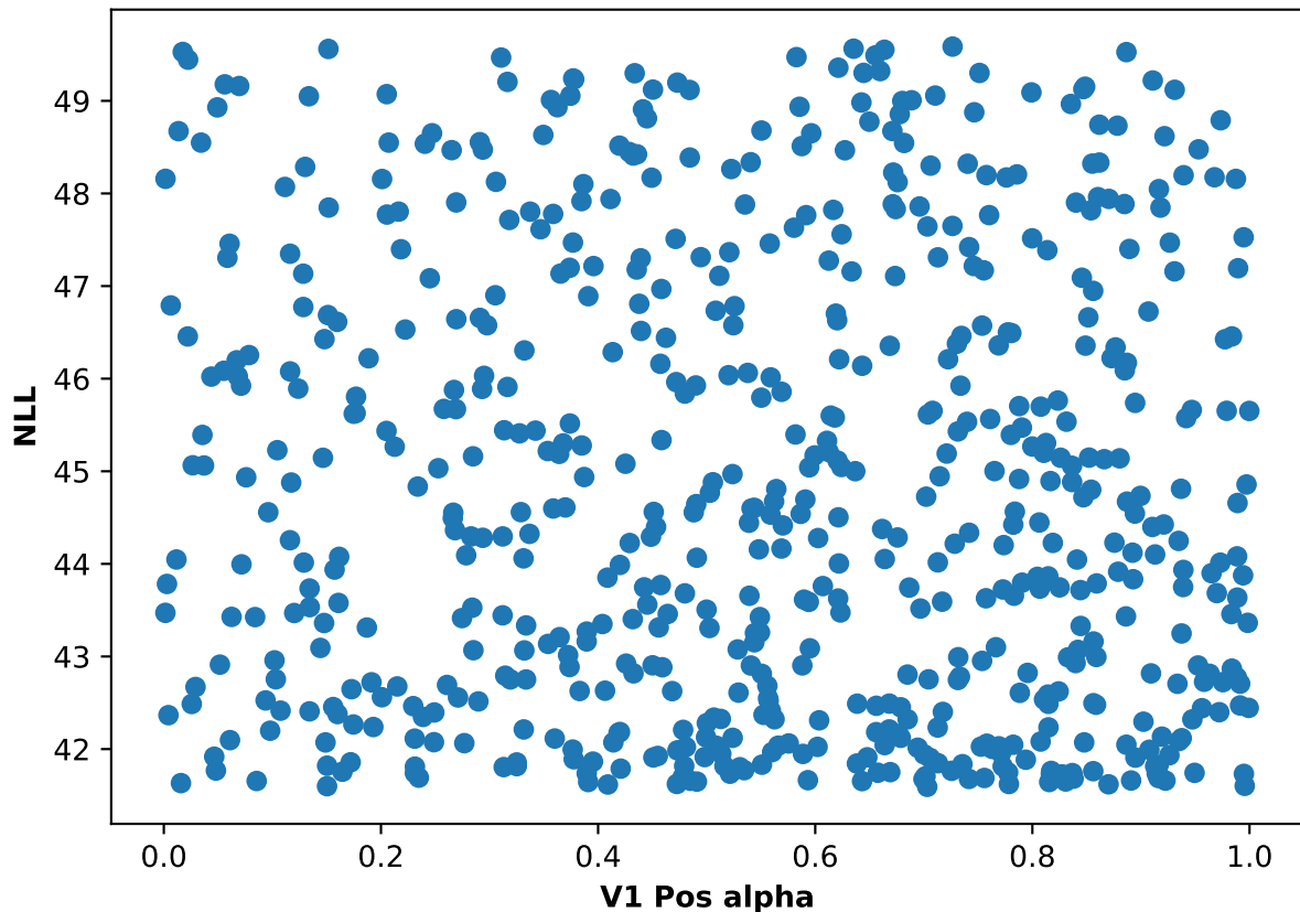
Participant 23, run 5: NLL and V1 Pos alpha scatter plot
