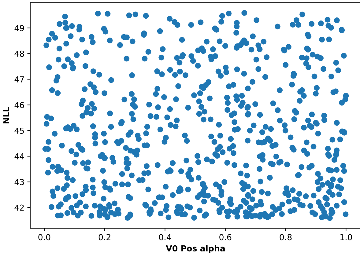
Participant 23, run 5: NLL and V0 Pos alpha scatter plot
