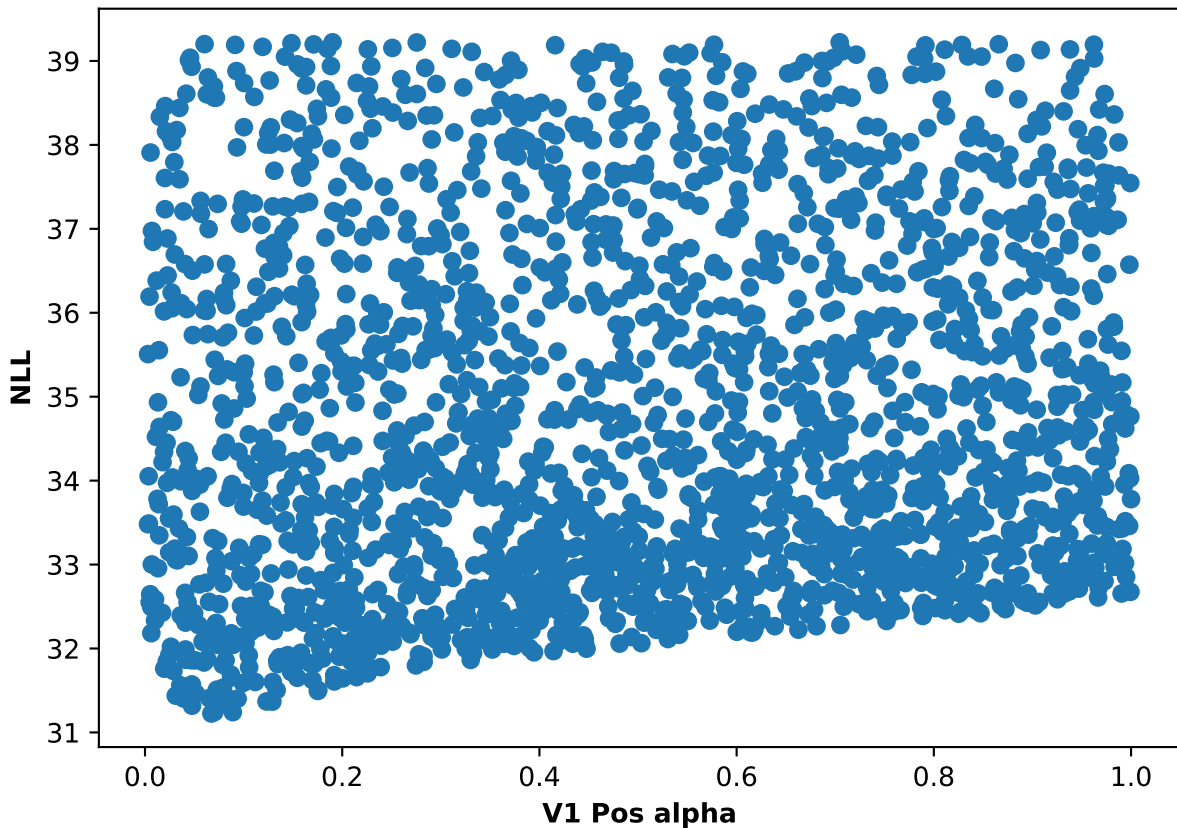
Participant 24, run 2: NLL and V1 Pos alpha scatter plot
