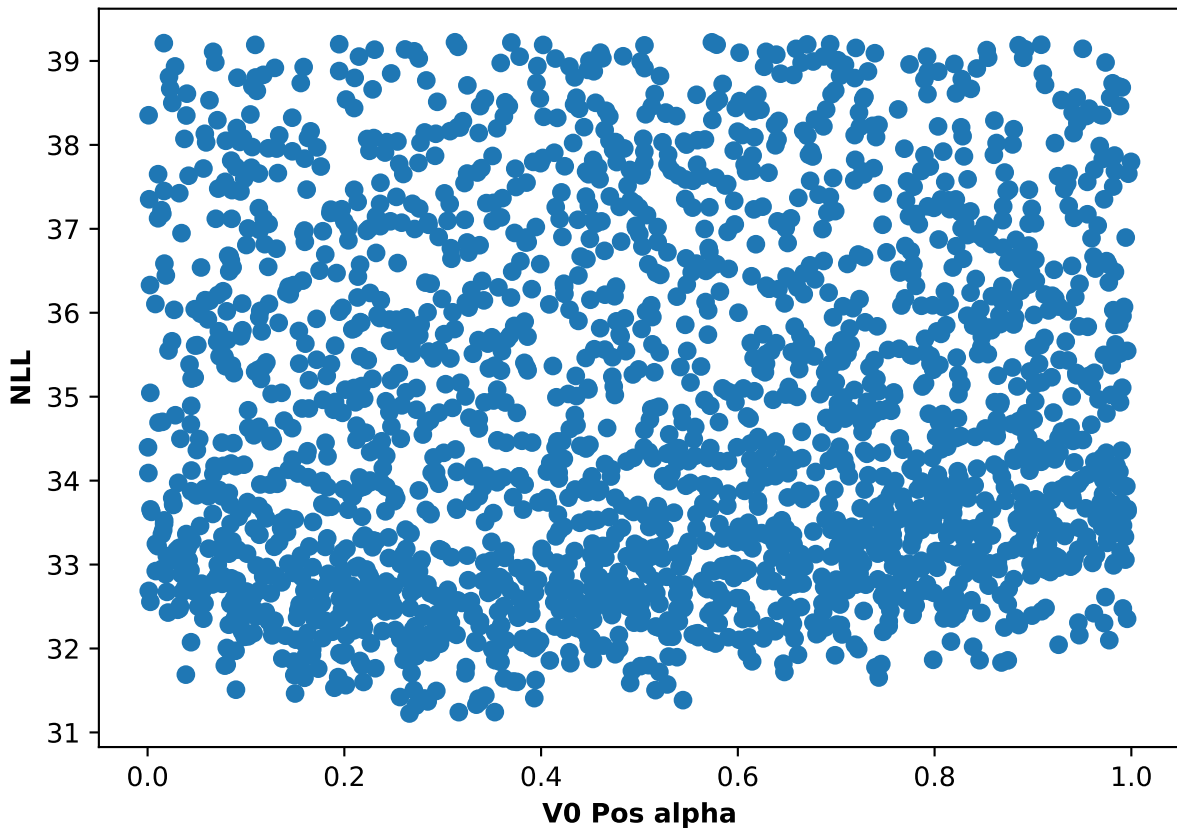
Participant 24, run 2: NLL and V0 Pos alpha scatter plot
