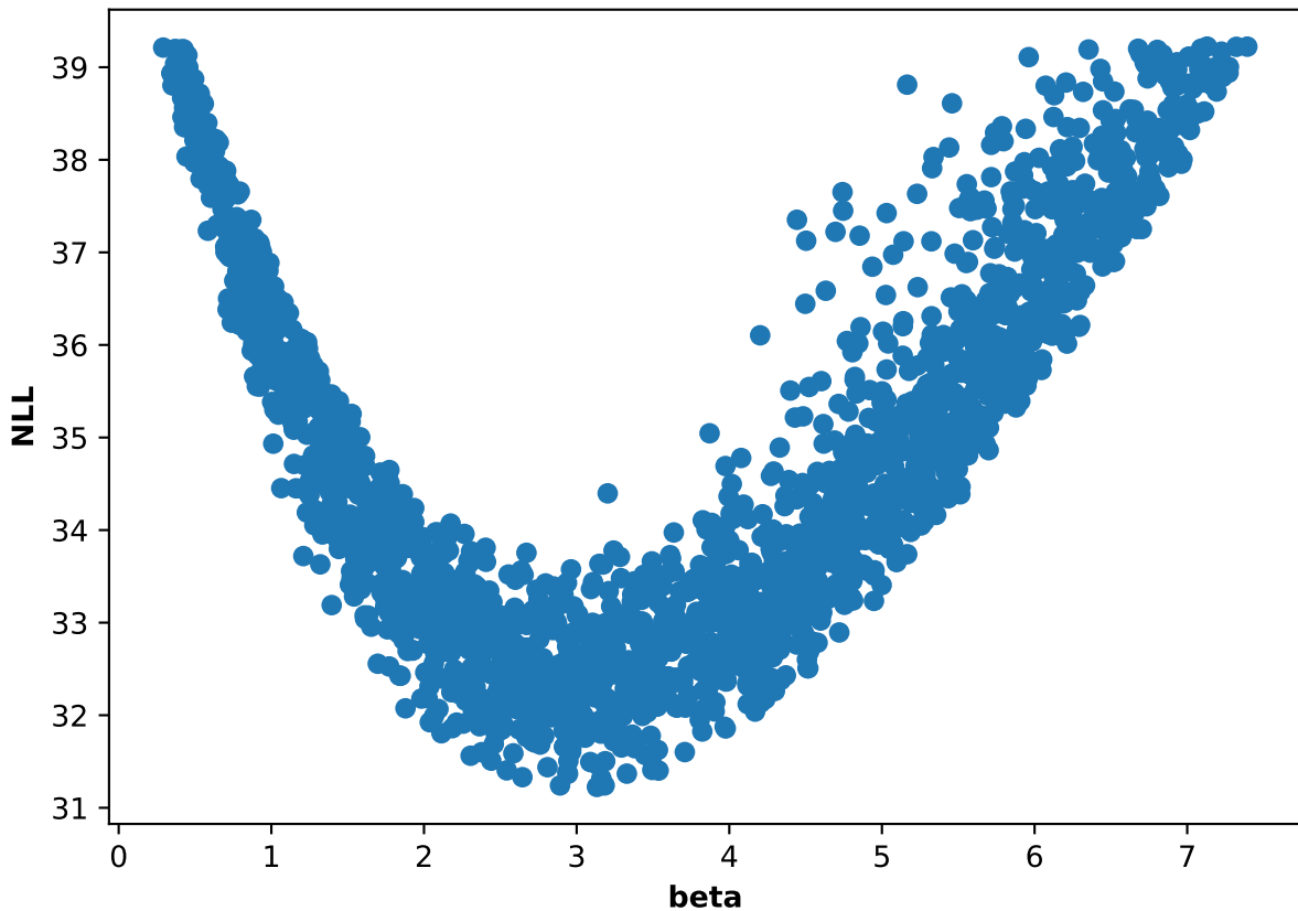
Participant 24, run 2: NLL and beta scatter plot
