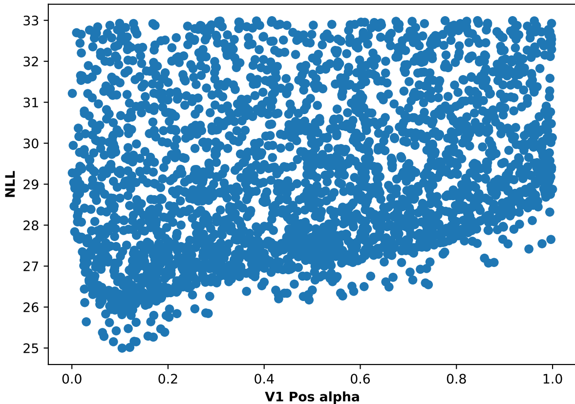
Participant 24, run 3: NLL and V1 Pos alpha scatter plot
