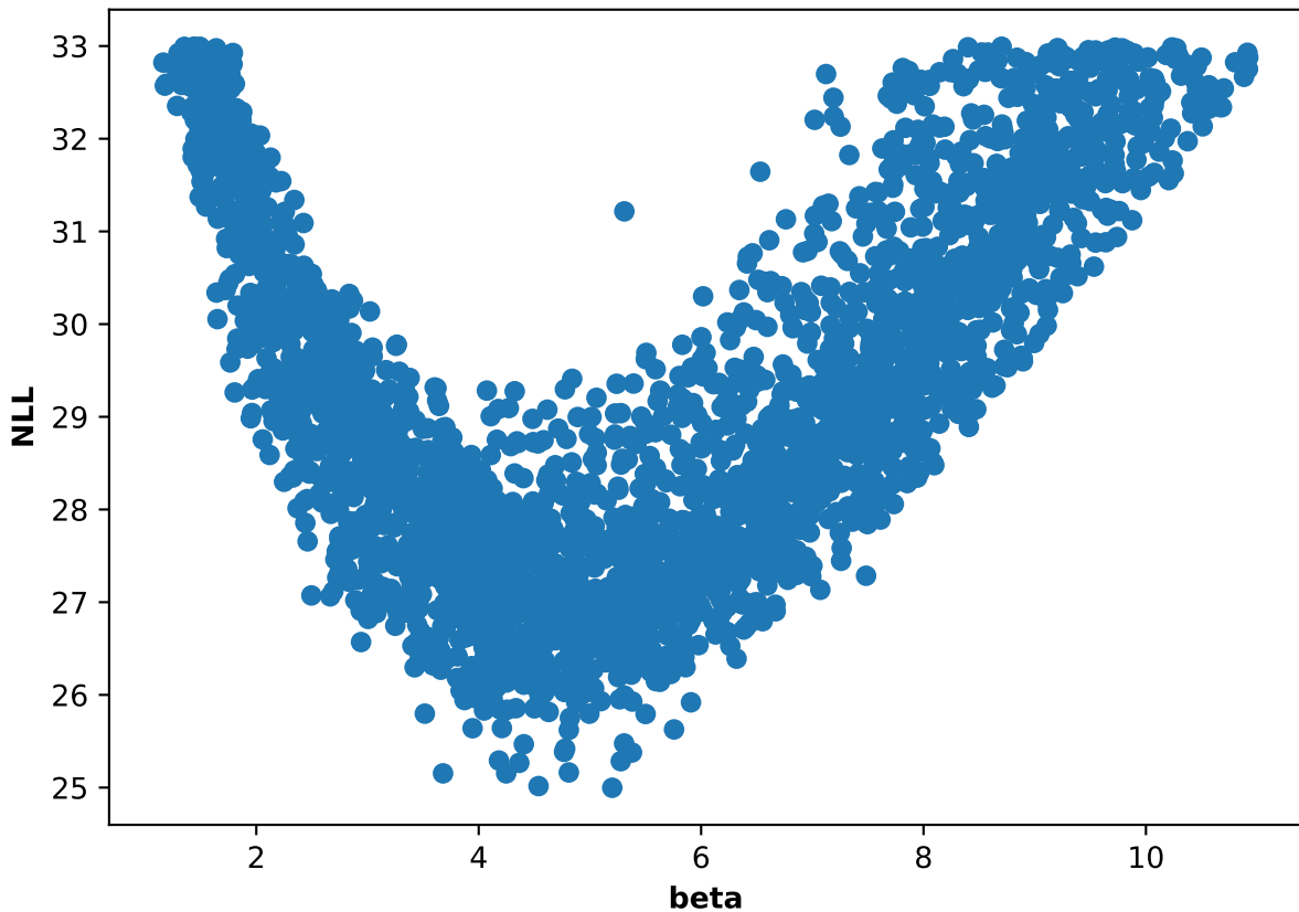
Participant 24, run 3: NLL and beta scatter plot
