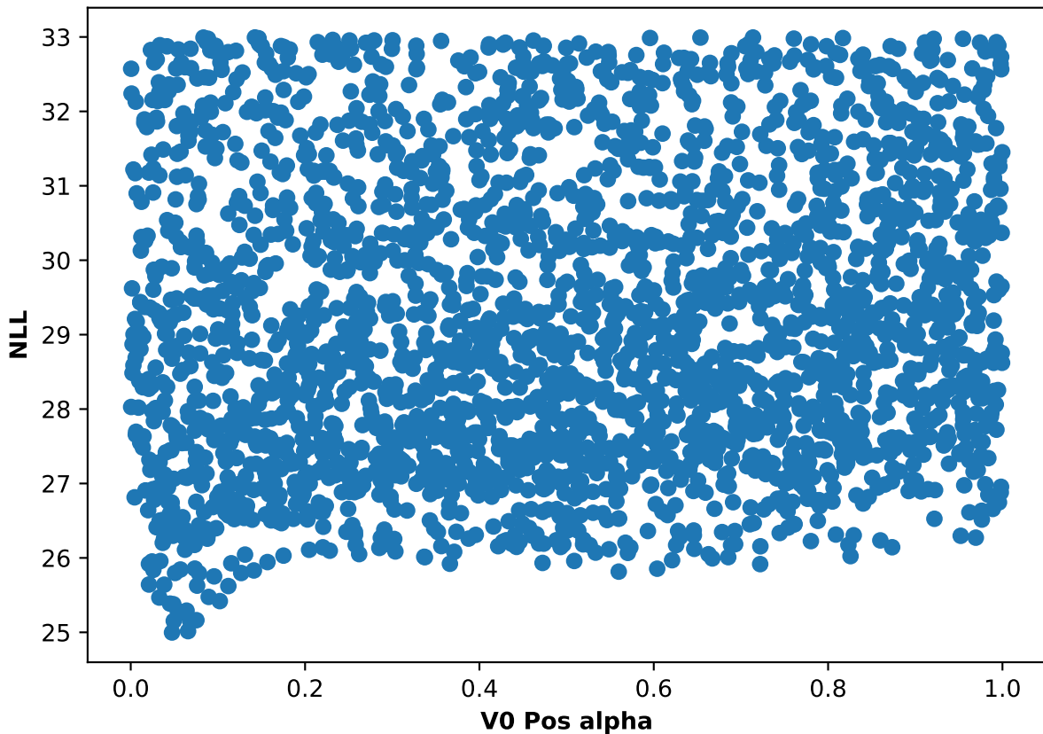
Participant 24, run 3: NLL and V0 Pos alpha scatter plot
