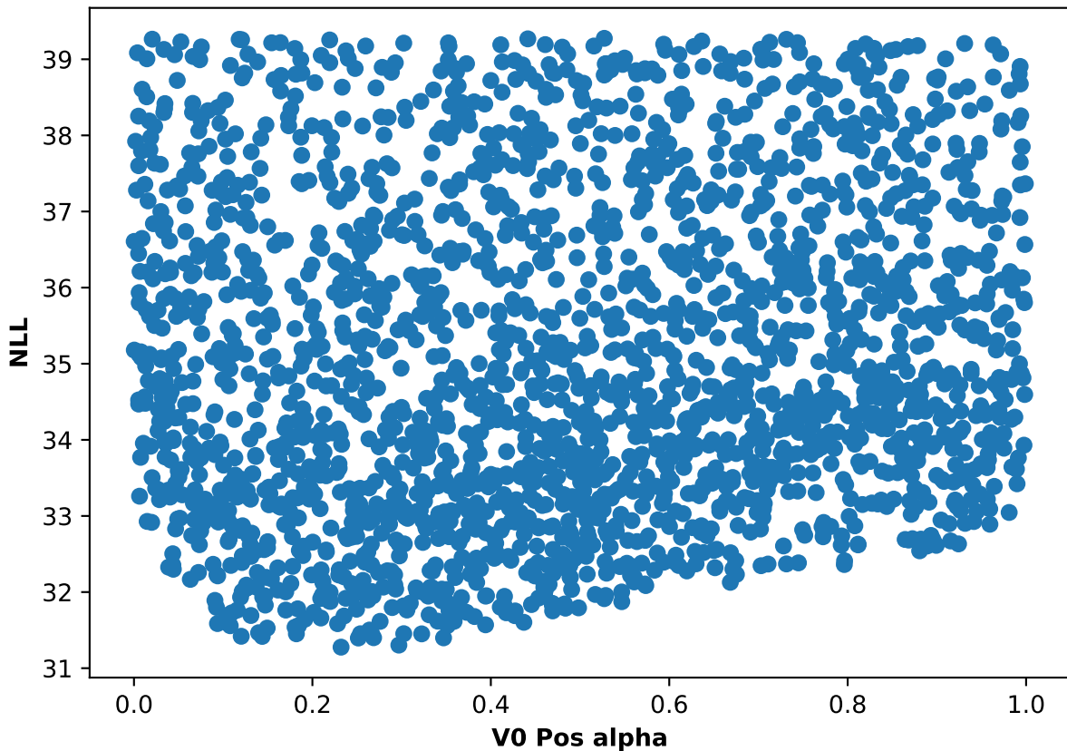
Participant 24, run 4: NLL and V0 Pos alpha scatter plot
