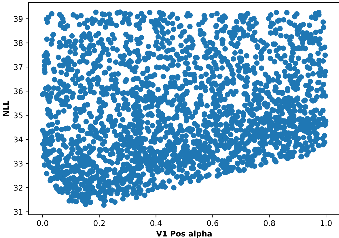
Participant 24, run 4: NLL and V1 Pos alpha scatter plot
