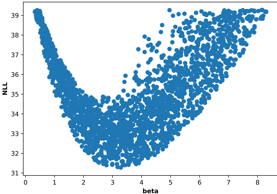
Participant 24, run 4: NLL and beta scatter plot
