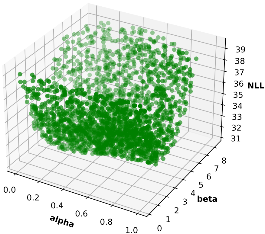
Participant 24, run 4: NLL, alpha and beta 3D scatter plot
