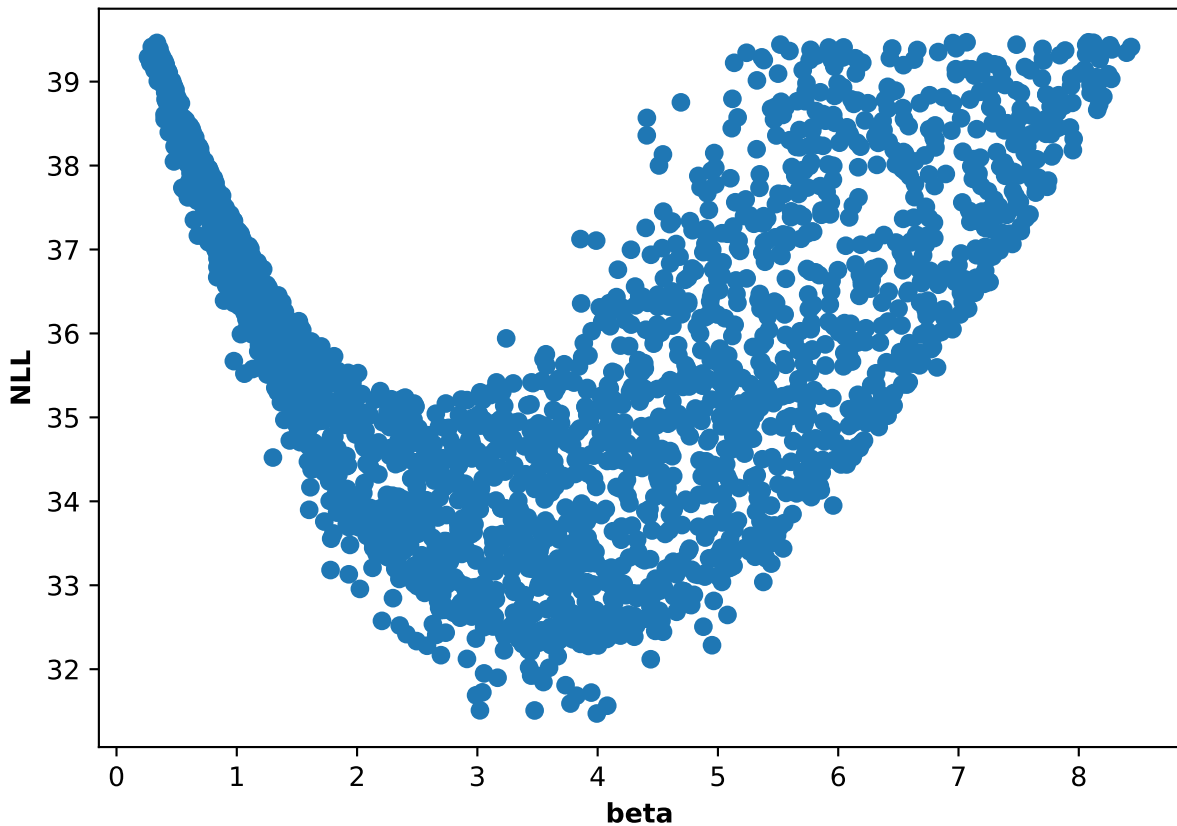
Participant 24, run 5: NLL and beta scatter plot
