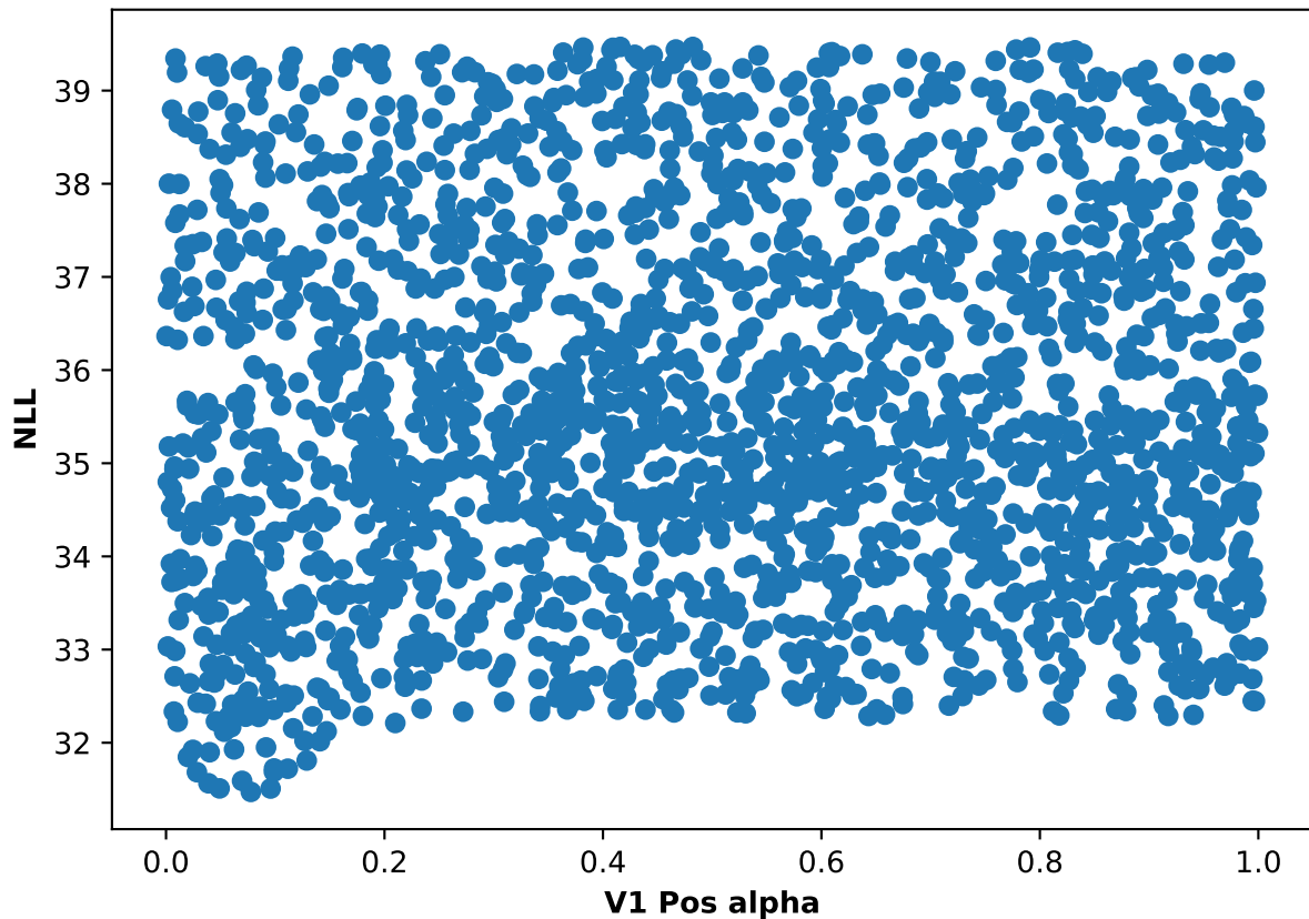
Participant 24, run 5: NLL and V1 Pos alpha scatter plot
