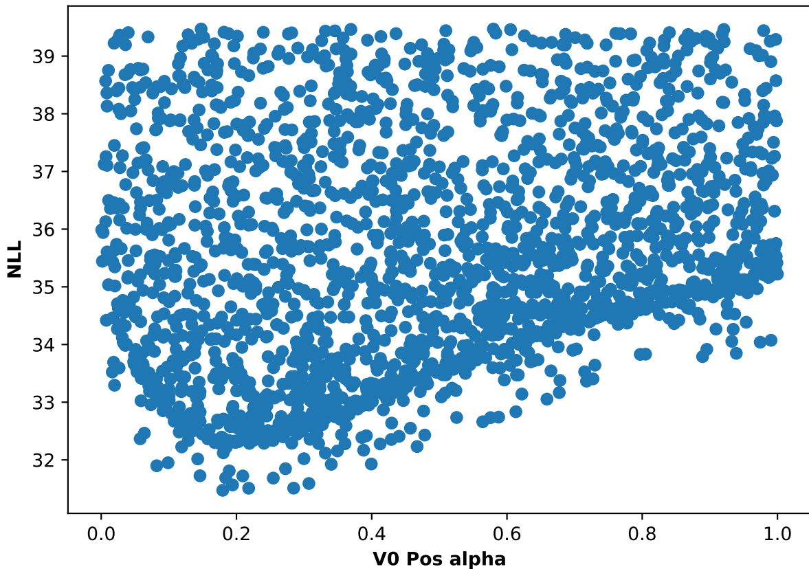
Participant 24, run 5: NLL and V0 Pos alpha scatter plot
