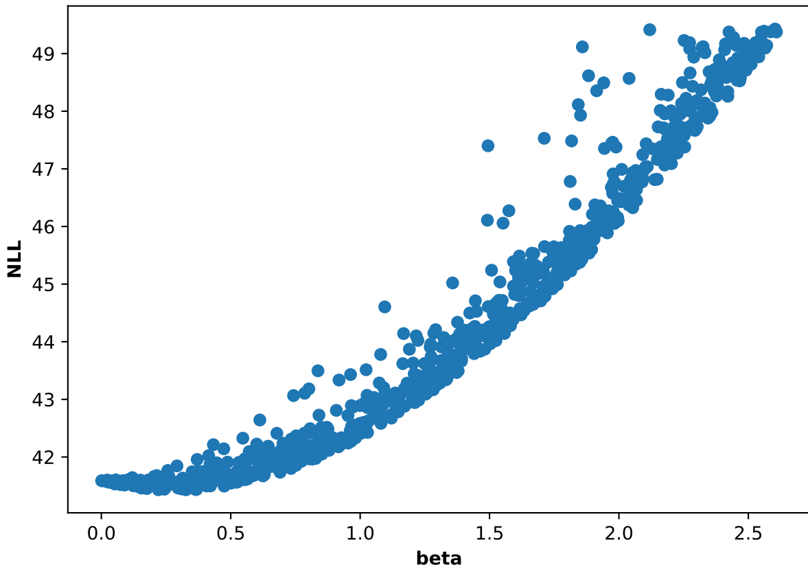
Participant 25, run 2: NLL and beta scatter plot
