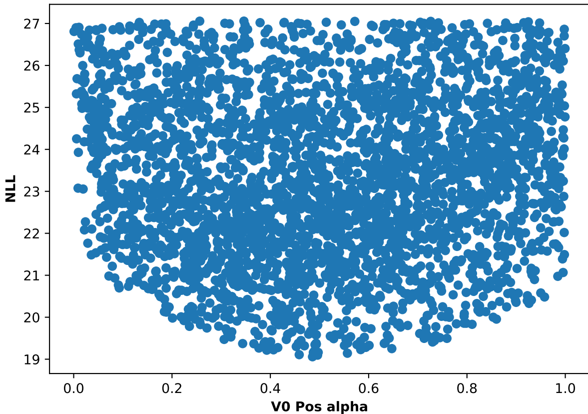
Participant 25, run 5: NLL and V0 Pos alpha scatter plot
