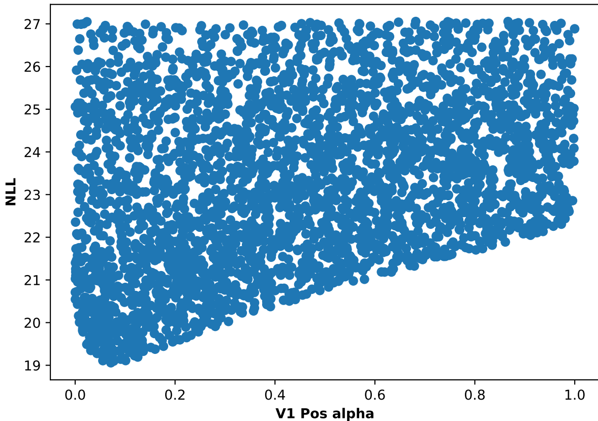
Participant 25, run 5: NLL and V1 Pos alpha scatter plot
