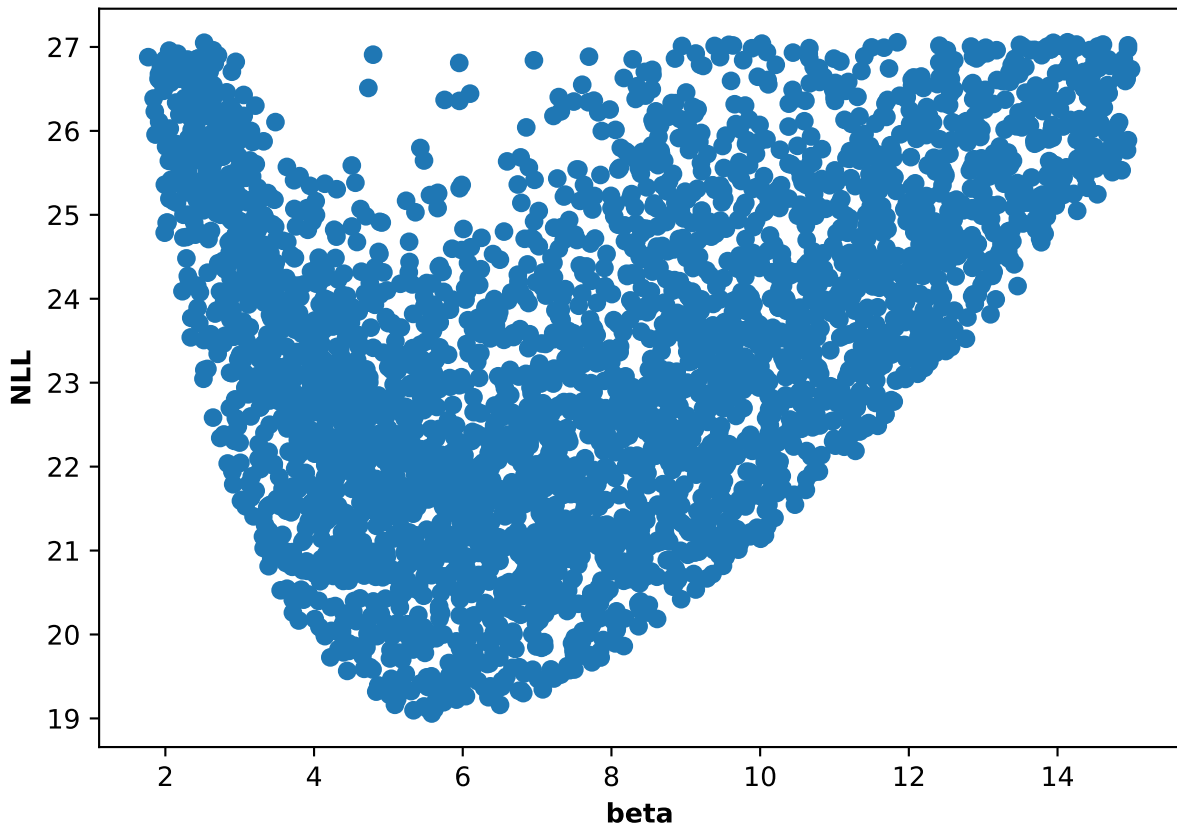
Participant 25, run 5: NLL and beta scatter plot
