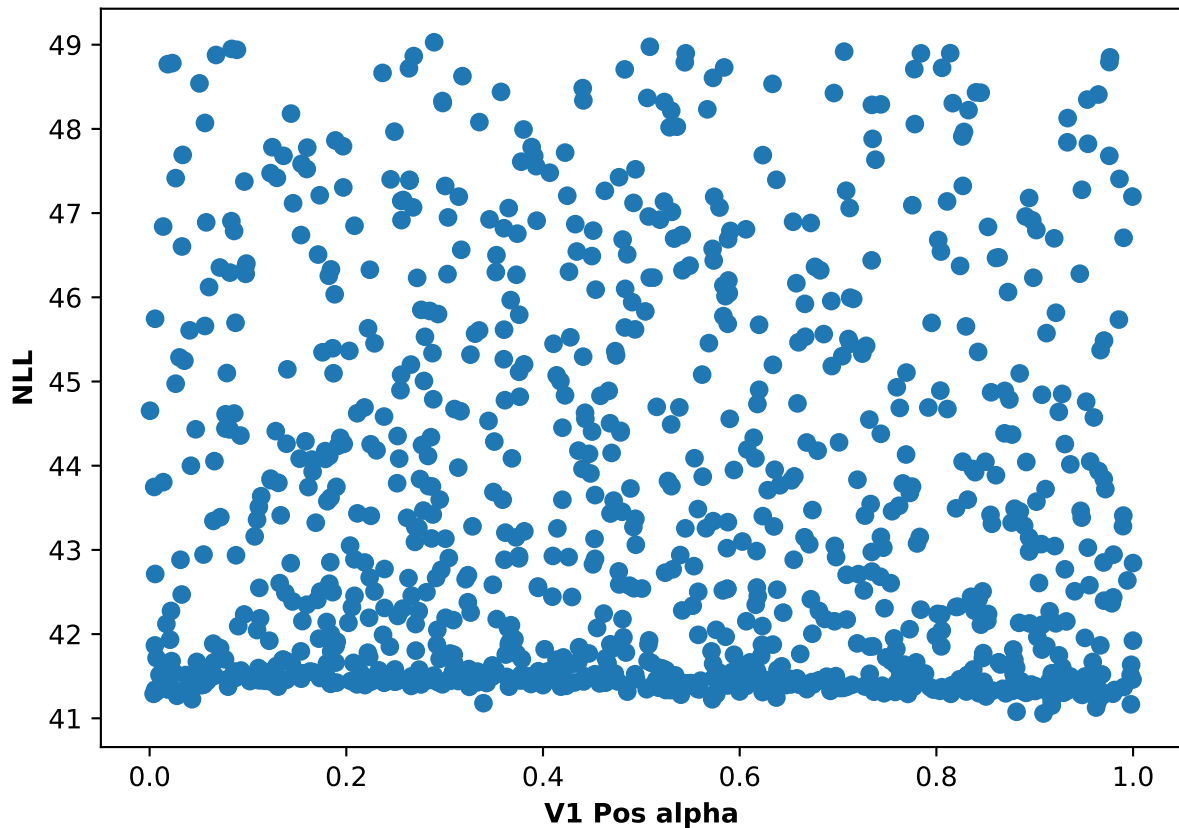
Participant 27, run 3: NLL and V1 Pos alpha scatter plot
