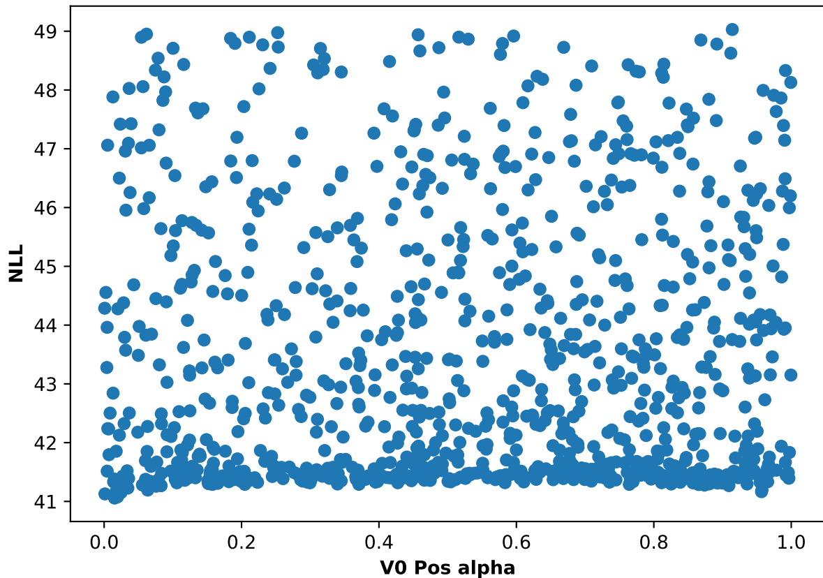
Participant 27, run 3: NLL and V0 Pos alpha scatter plot
