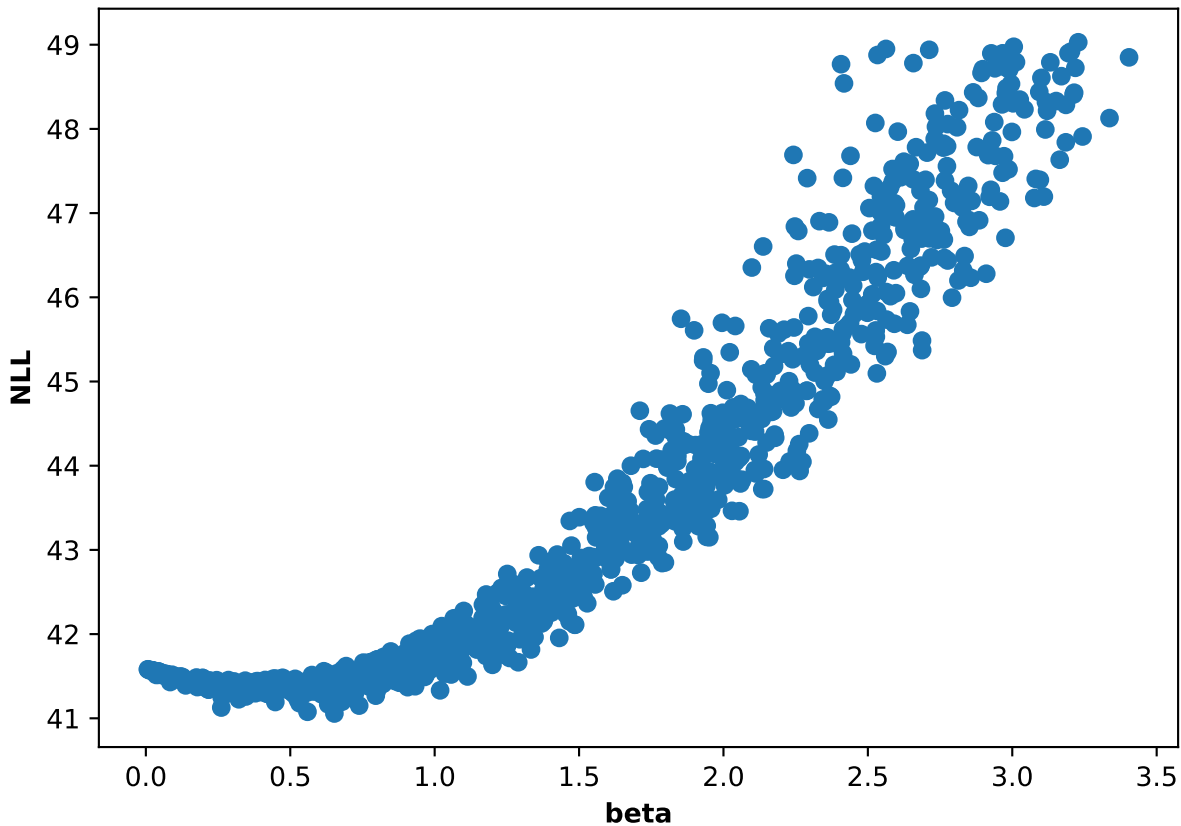
Participant 27, run 3: NLL and beta scatter plot
