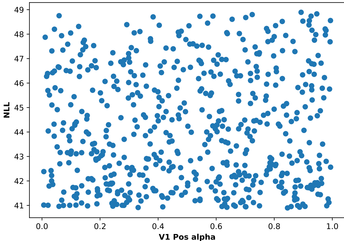
Participant 27, run 5: NLL and V1 Pos alpha scatter plot
