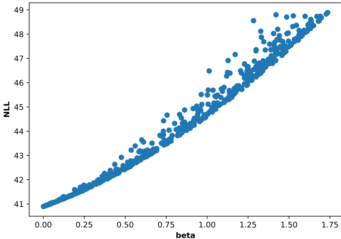
Participant 27, run 5: NLL and beta scatter plot
