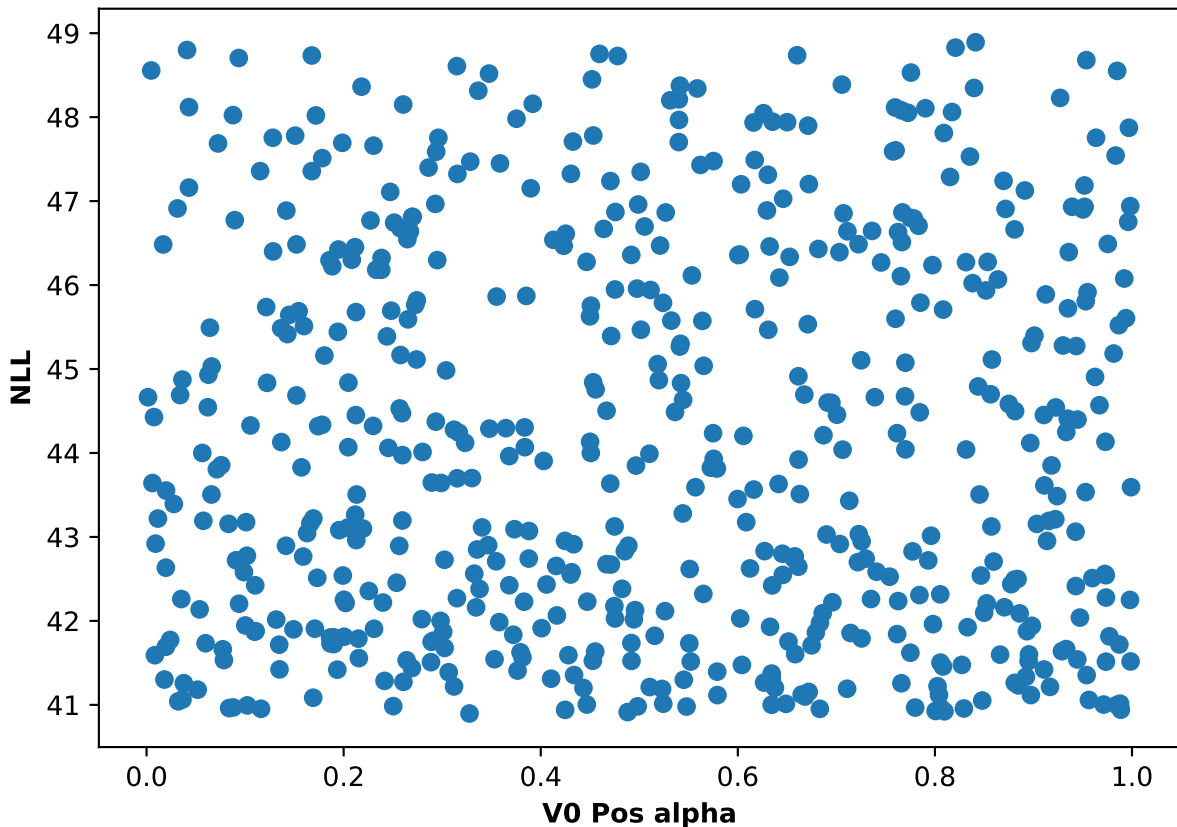
Participant 27, run 5: NLL and V0 Pos alpha scatter plot
