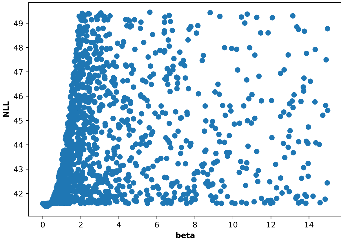
Participant 28, run 1: NLL and beta scatter plot
