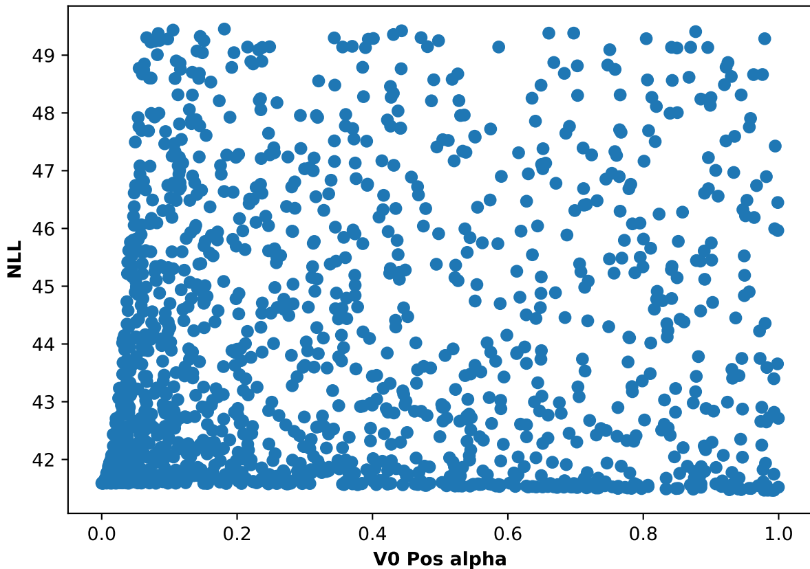
Participant 28, run 1: NLL and V0 Pos alpha scatter plot
