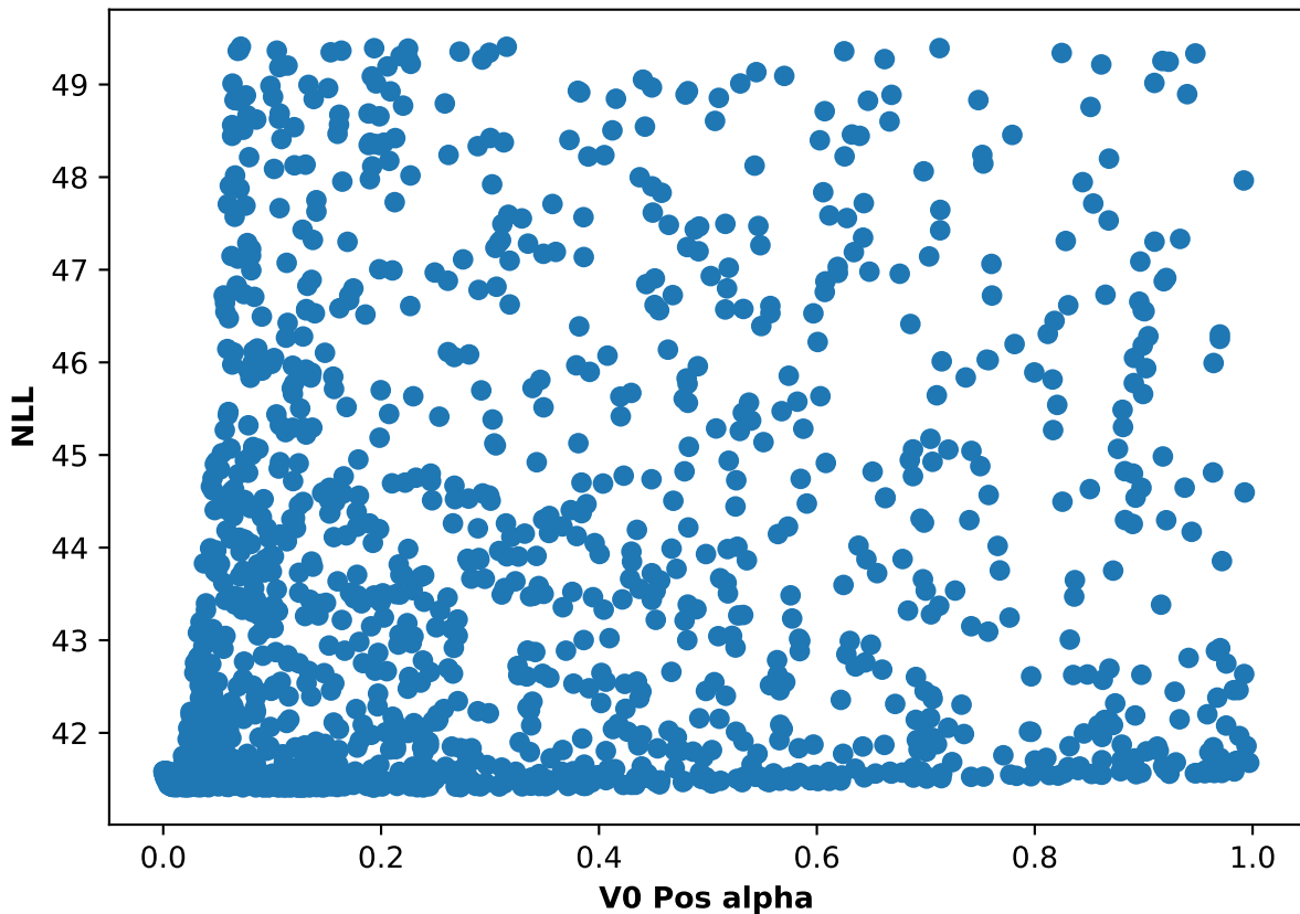
Participant 28, run 2: NLL and V0 Pos alpha scatter plot
